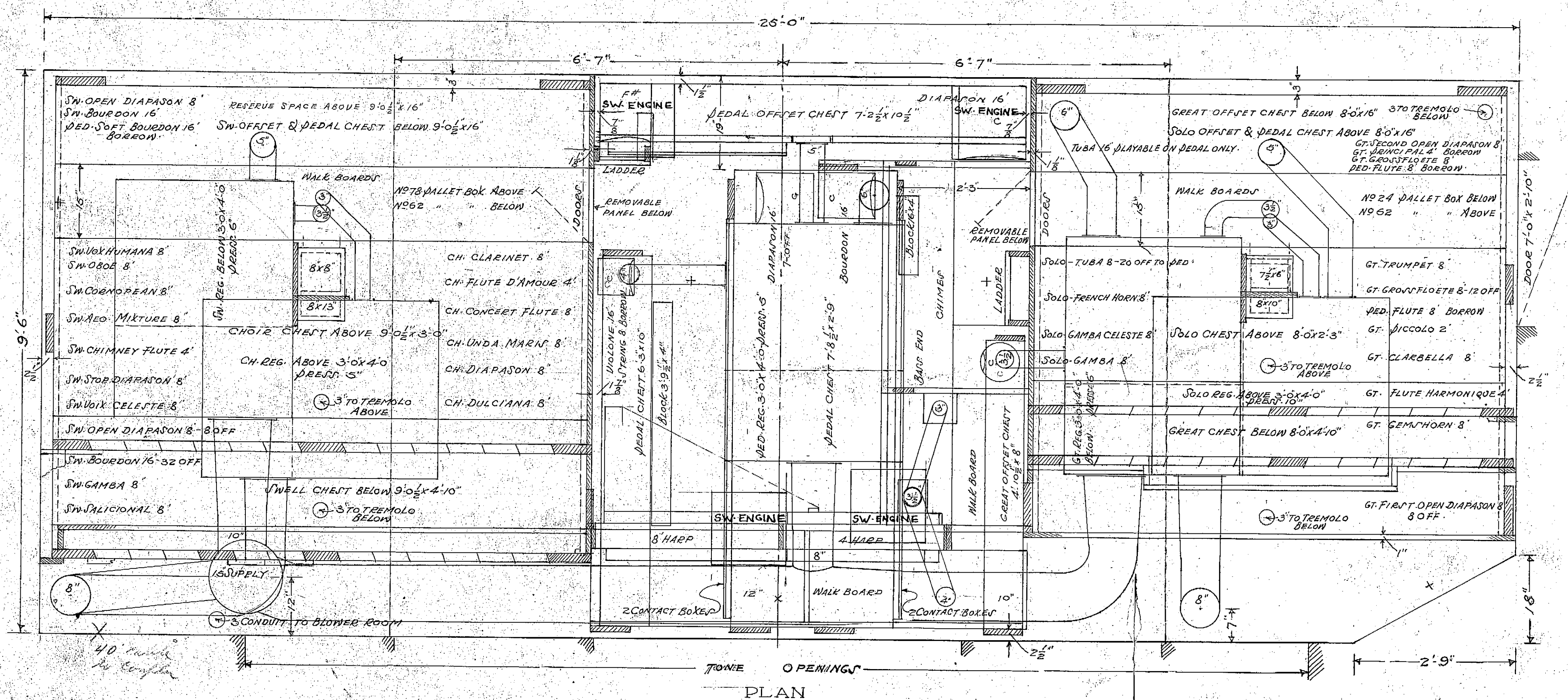
PLAN
