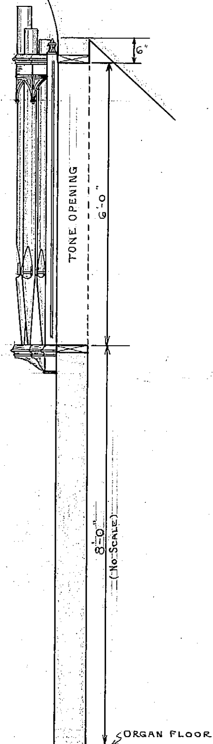
CROSS SECTION
