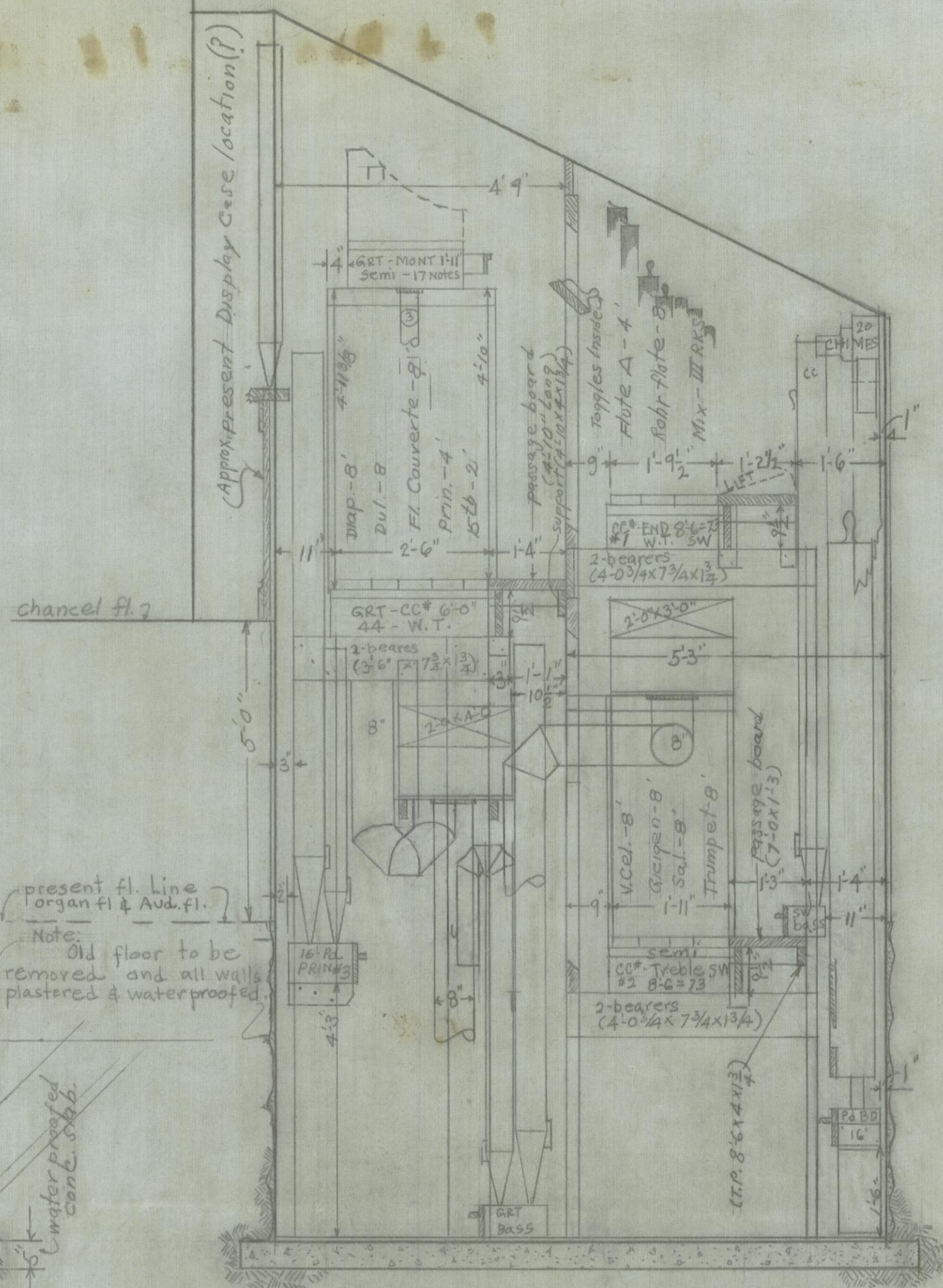
SECTION C-C
