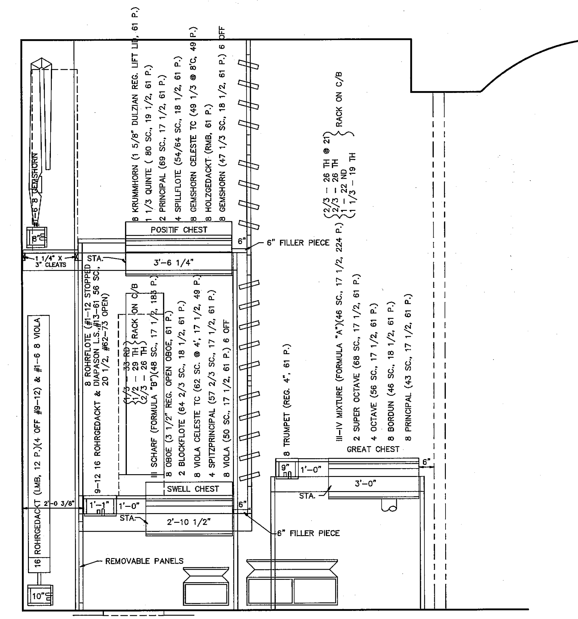
SECTION BB
