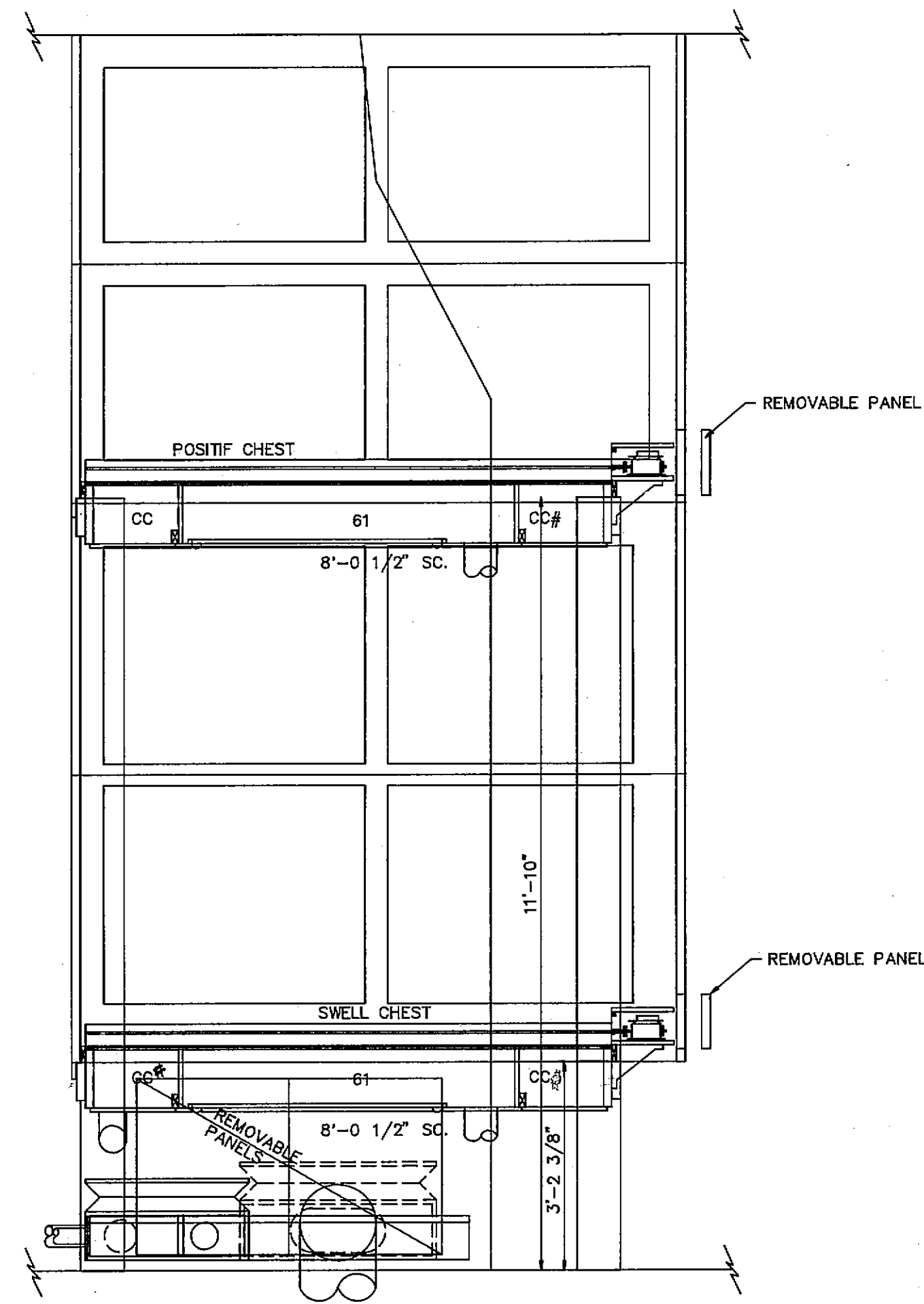
SECTION CC
