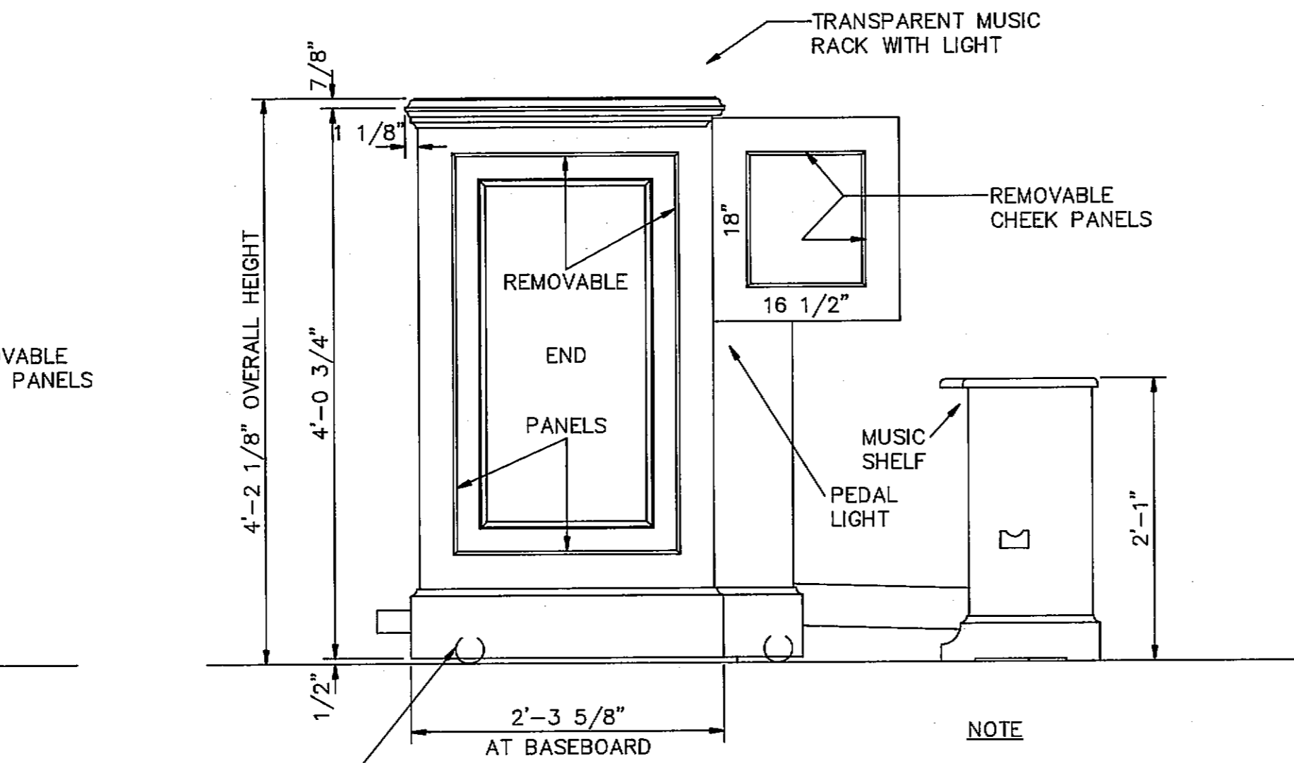
END VIEW
