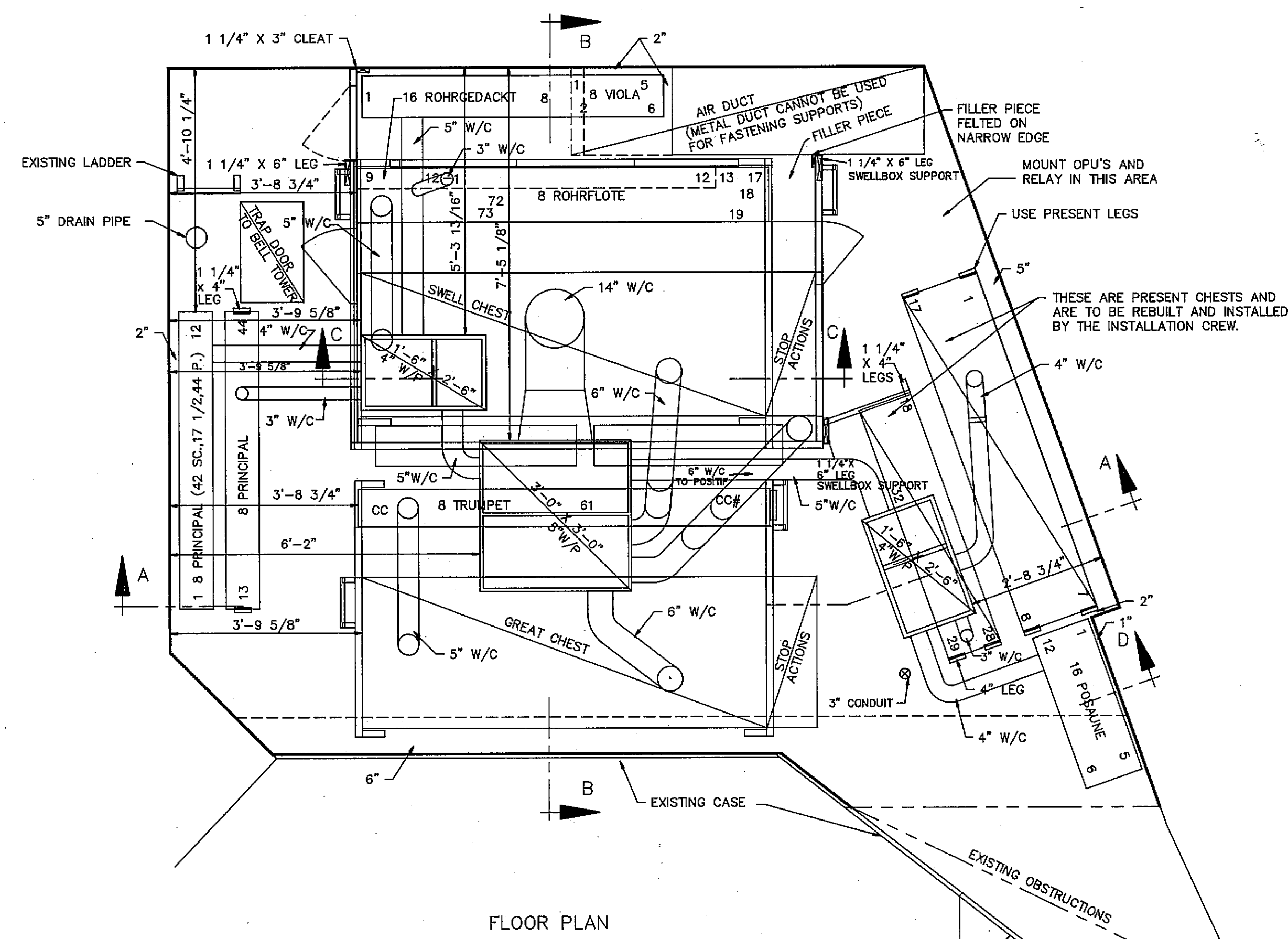
FLOOR PLAN
