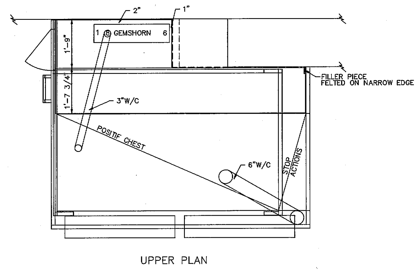
UPPER PLAN
