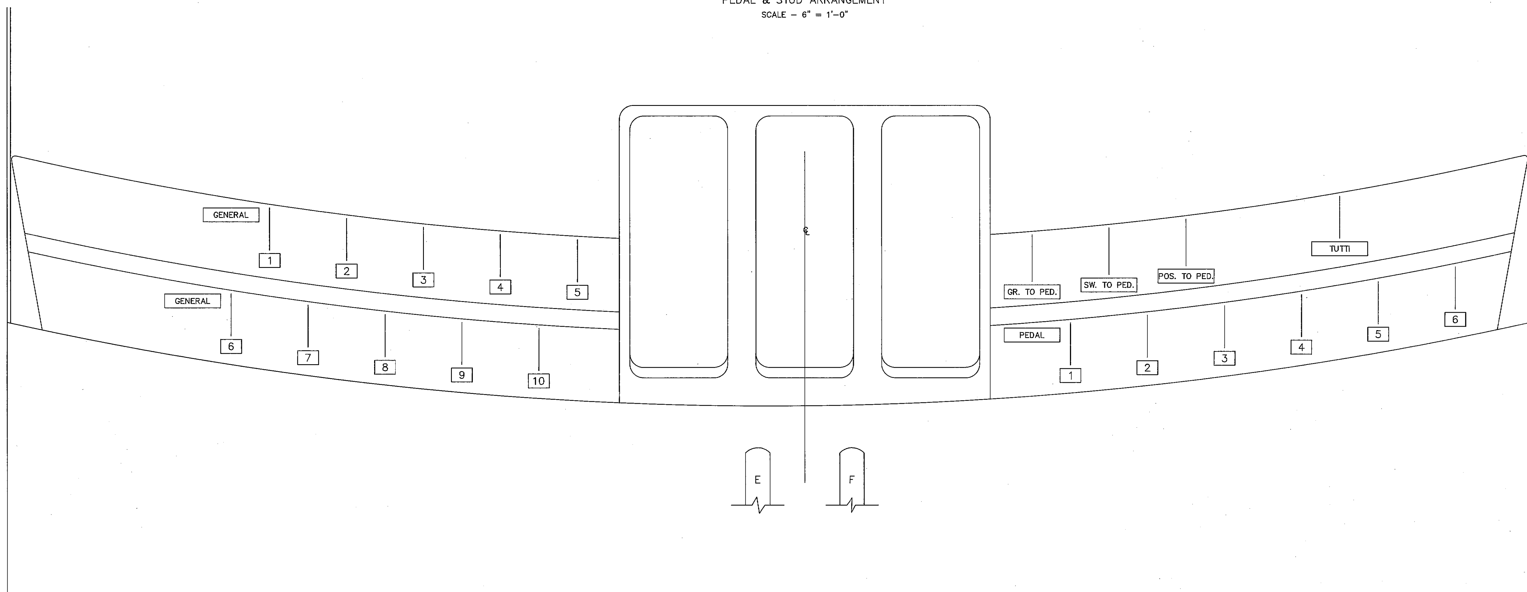
PEDAL & STUD ARRANGEMENT SCALE - 6" = 1'-0"
