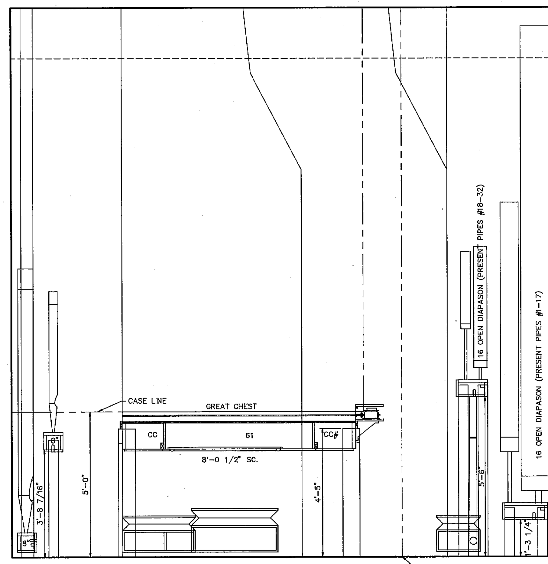
SECTION AA
