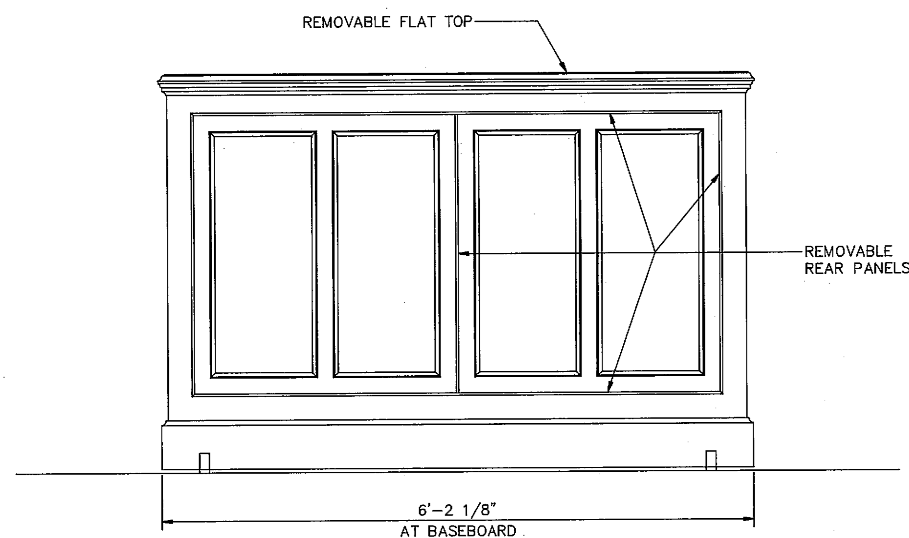
REAR VIEW
