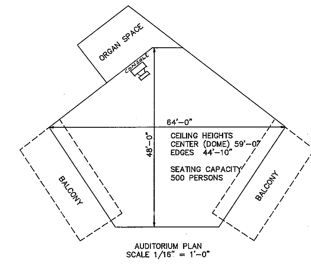
AUDITORIUM PLAN SCALE 1/16" = 1'-0"
