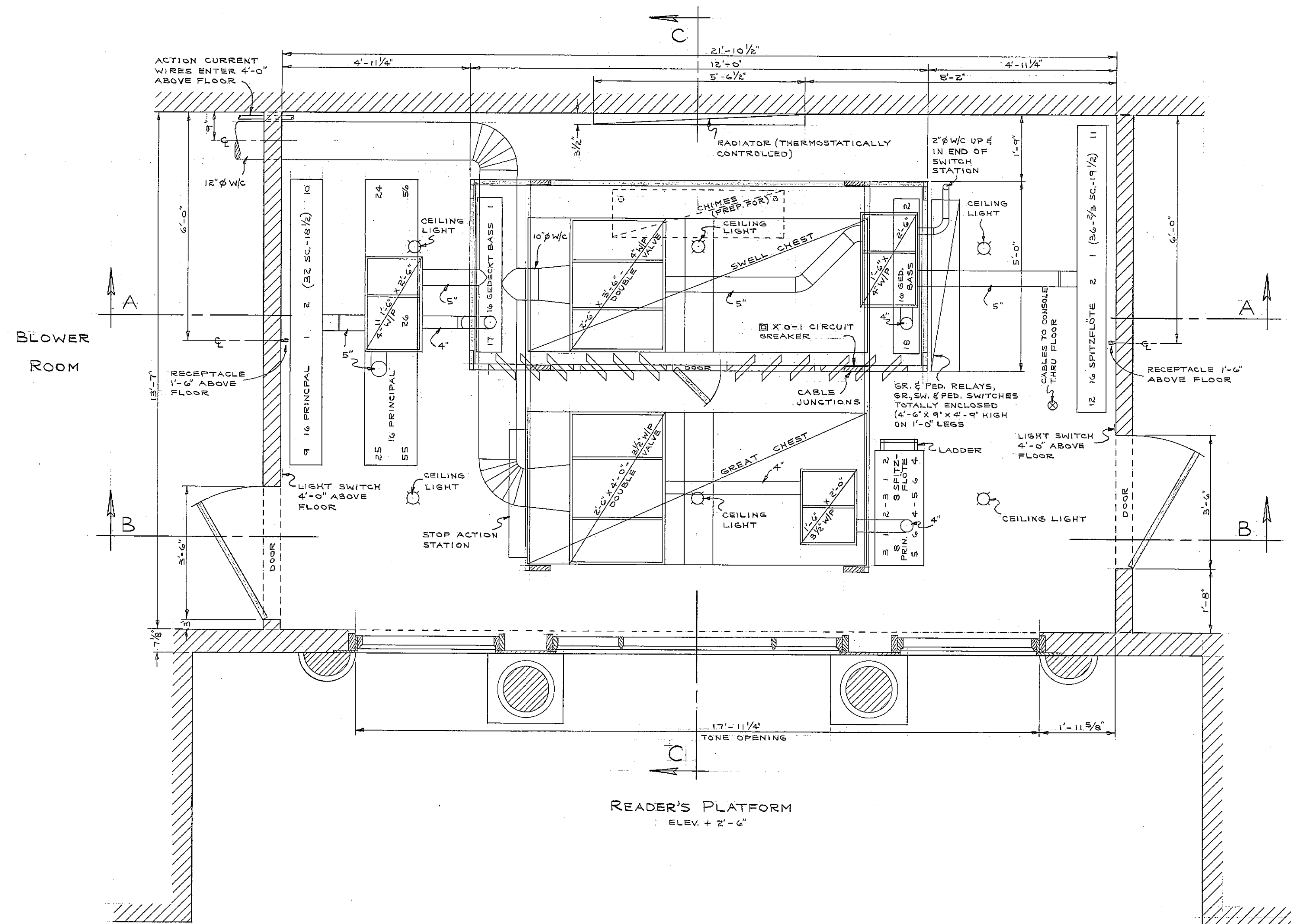
FLOOR PLAN
