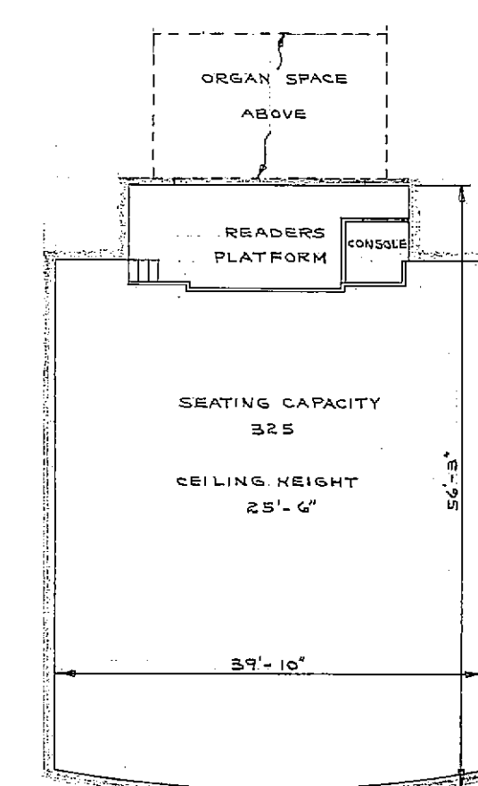
AUDITORIUM PLAN
