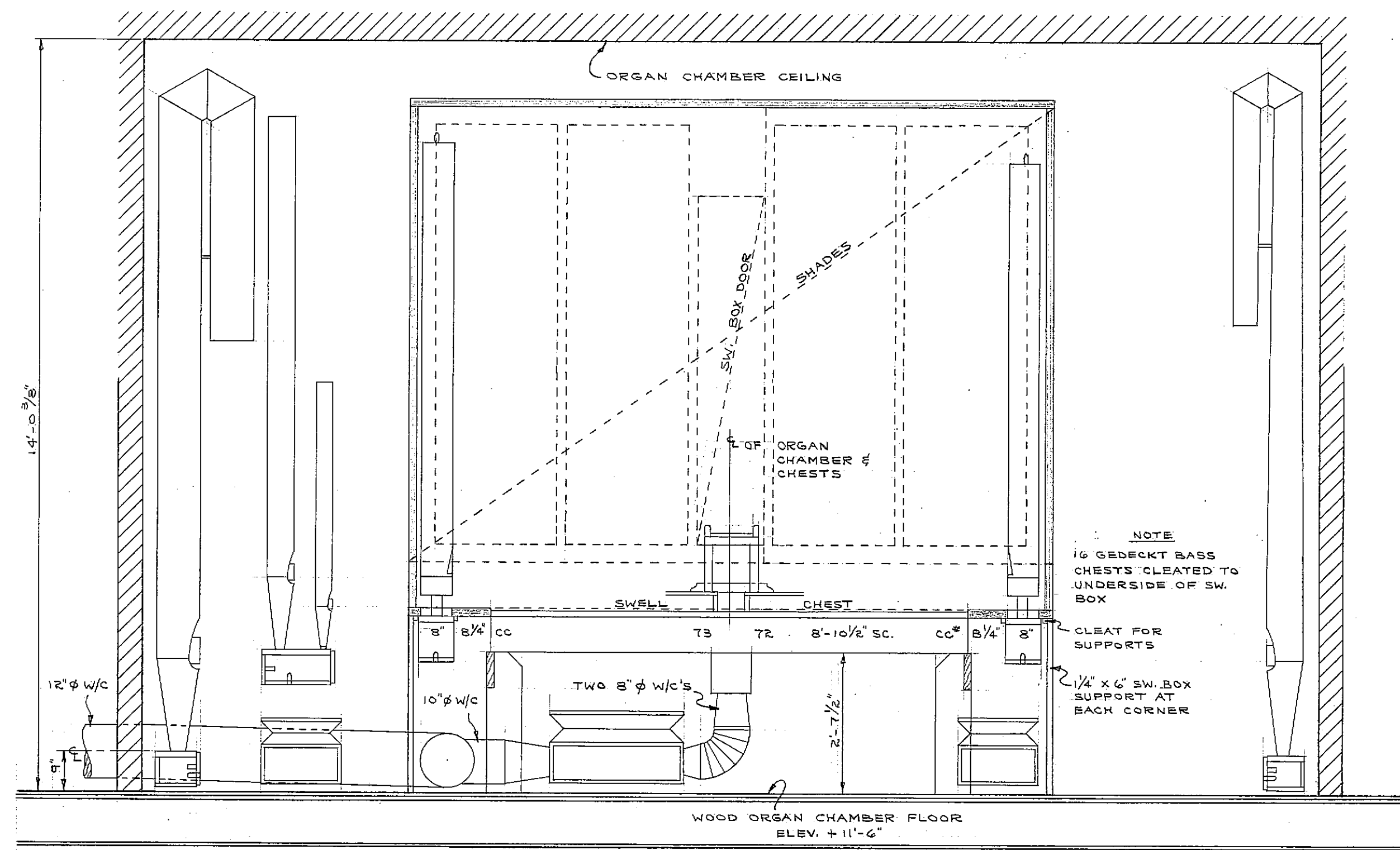
SECTION AA
