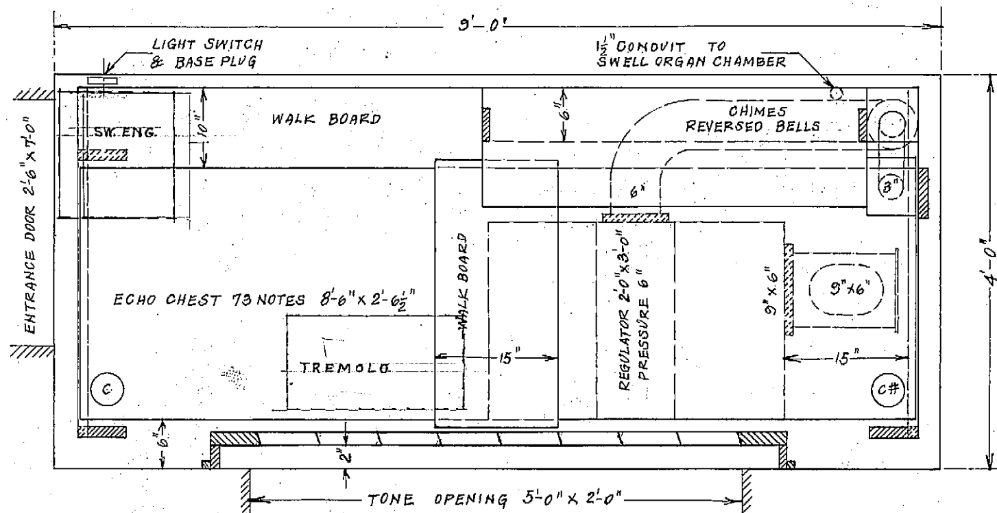
PLAN
