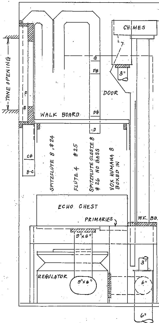
SECTION
