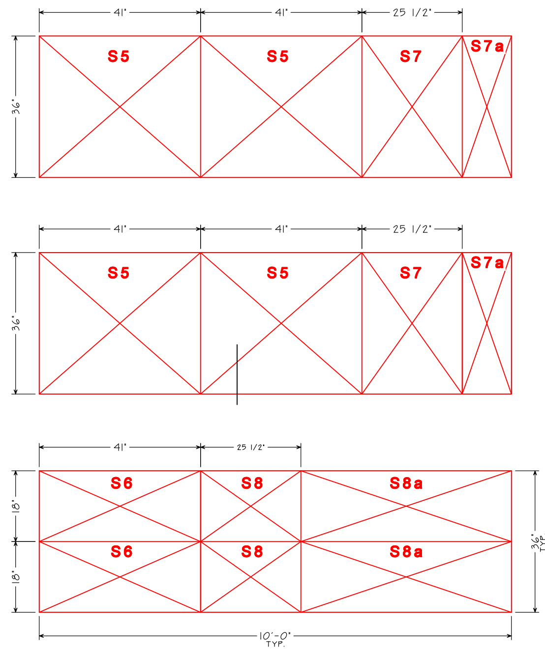
WIRE CUT PATTERNS
