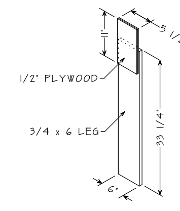
LEG G DETAIL
