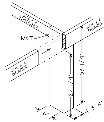
LEG B DETAIL
