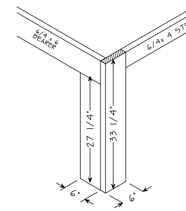
LEG F DETAIL
