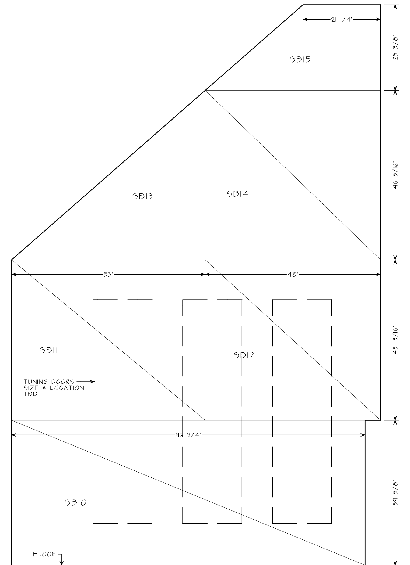
4 9 SW BOX PANEL DETAIL AT SWELL LEFT END SCALE 3/4" = 1' 0"
