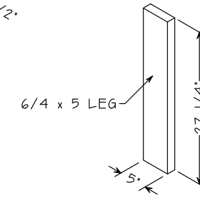
LEG J DETAIL
