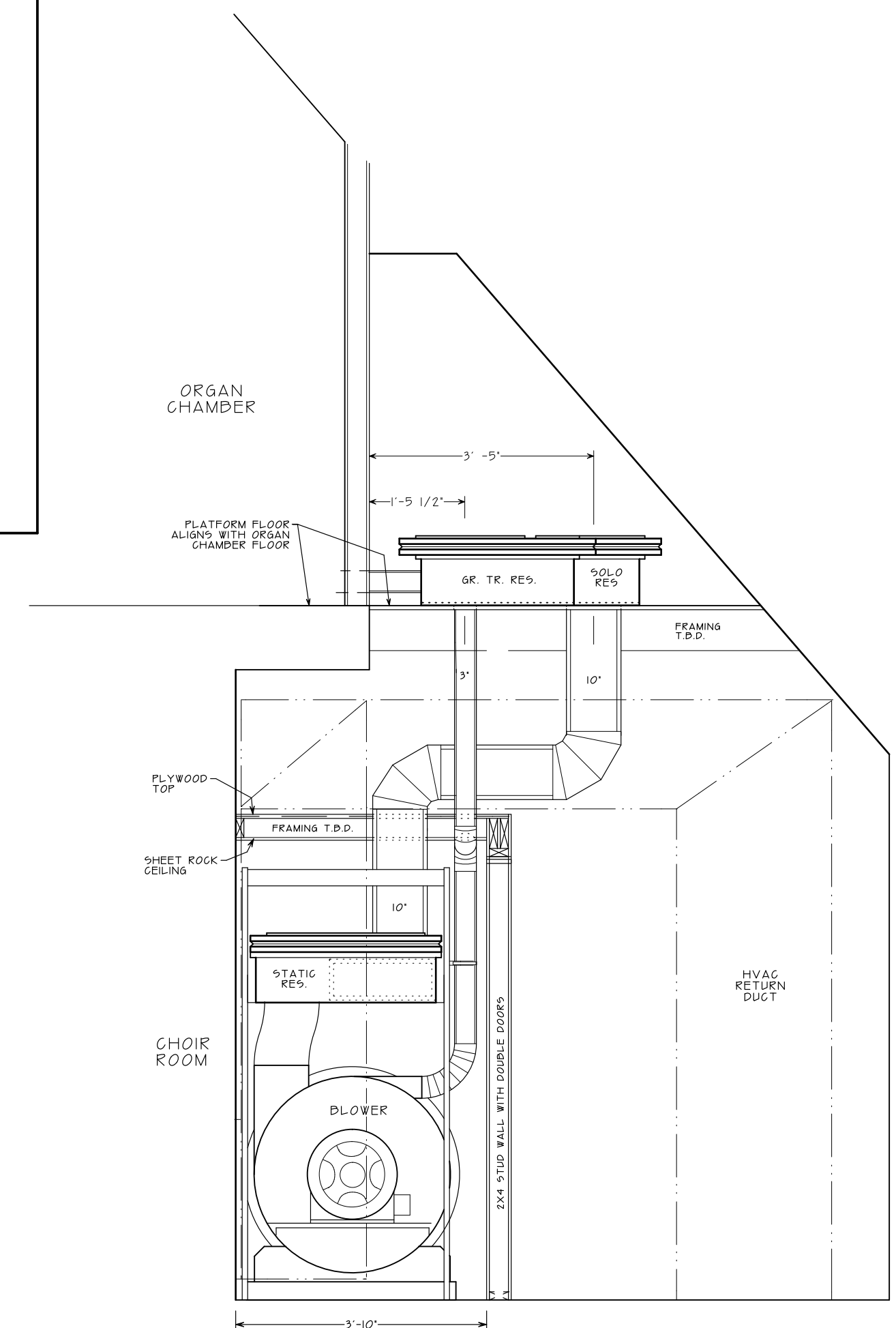
2/12 BLOWER/WINDING SECTION
