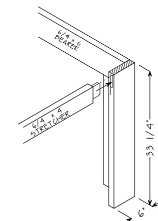
LEG H DETAIL
