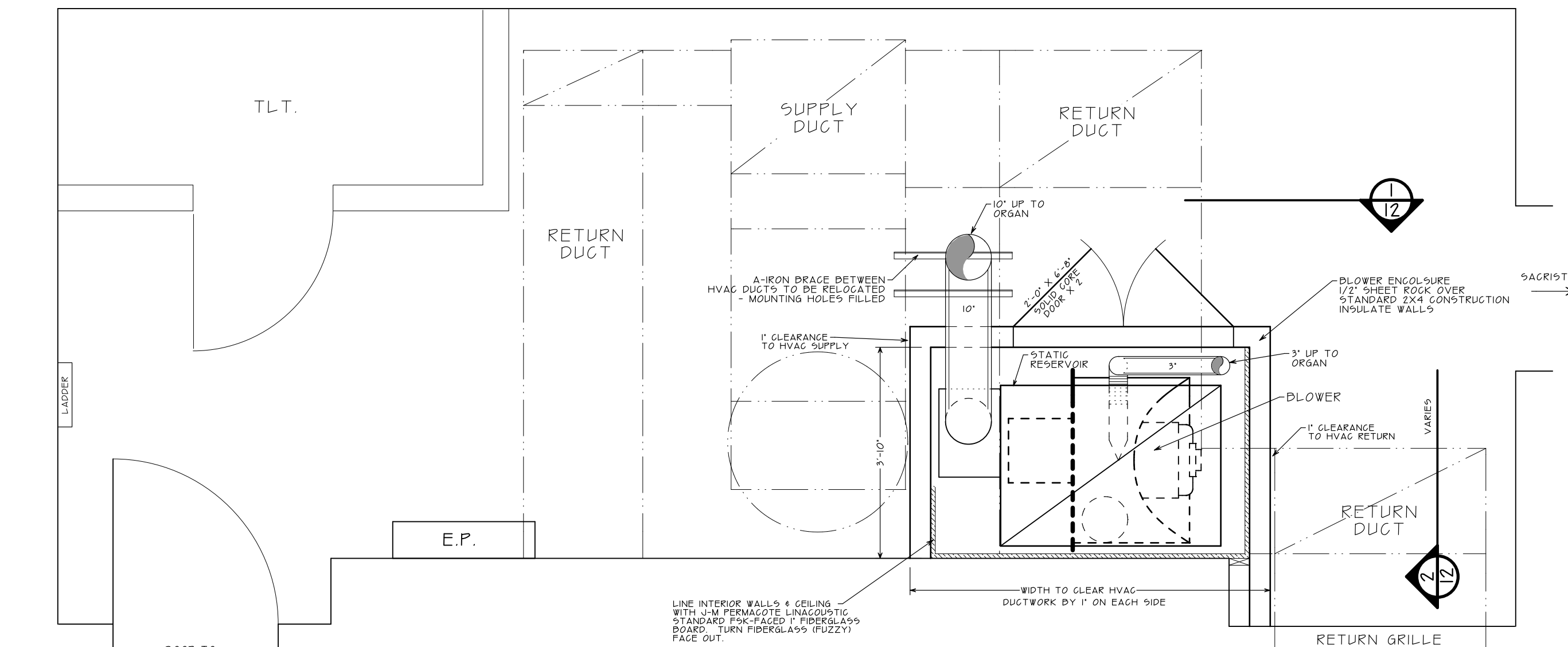
MECHANICAL ROOM PLAN
