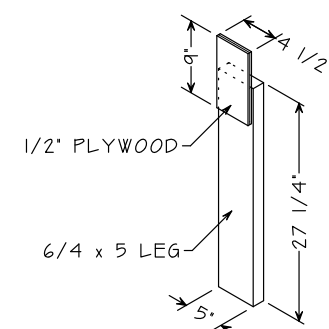
LEG I DETAIL
