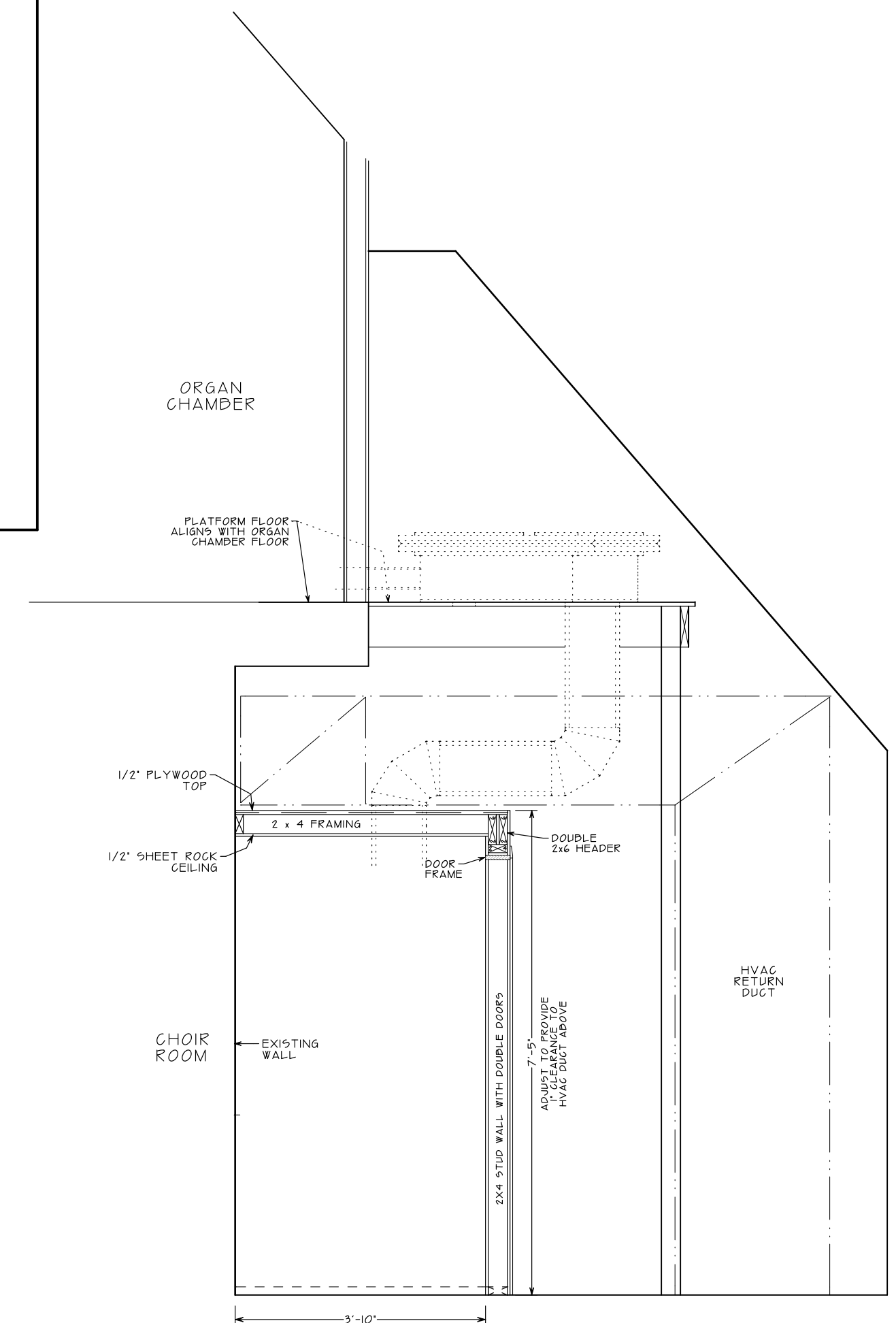
BLOWER ENCLOSURE SECTION
