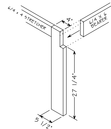
LEG E DETAIL
