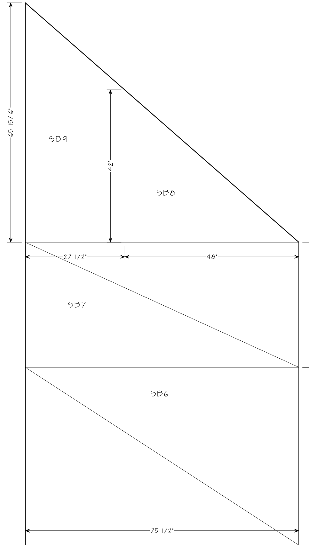
3 9 SW BOX PANEL DETAIL AT SOLO RIGHT END SCALE 3/4" = 1' 0"
