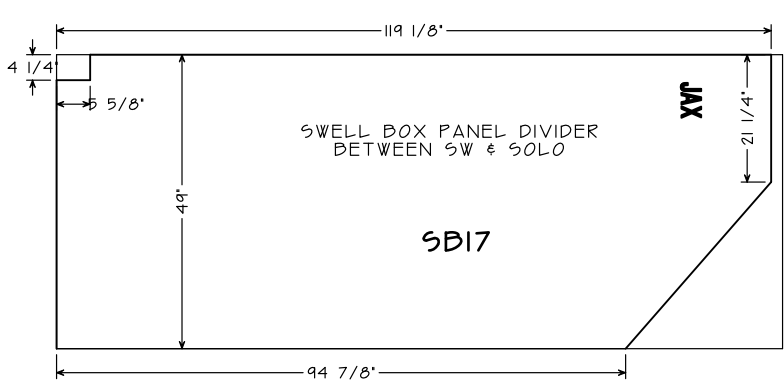
MDF 49 x 121 CUT SHEETS SCALE 3/8" = 1' 0"
