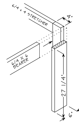
LEG D DETAIL
