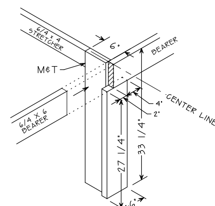
LEG K DETAIL
