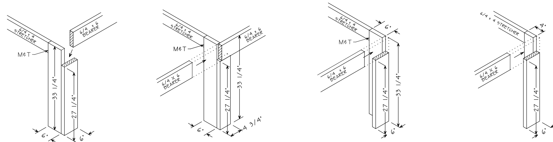
LEG A DETAIL
