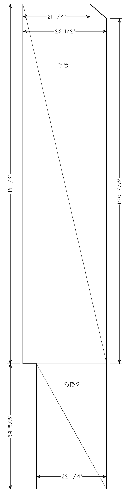
2 9 SW BOX PANEL DETAIL AT SOLO INTERMEDIATE SCALE 3/4" = 1' 0"
