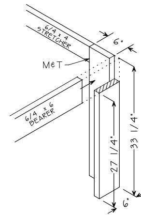
LEG C DETAIL
