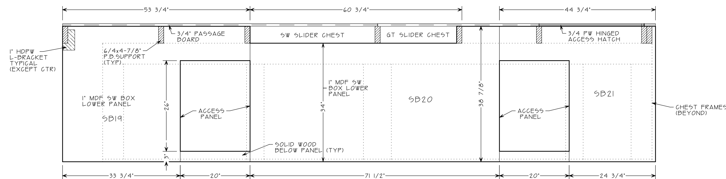
1 9 SW BOX PANEL DETAIL AT LOWER LEVEL SCALE 3/4" = 1' 0"
