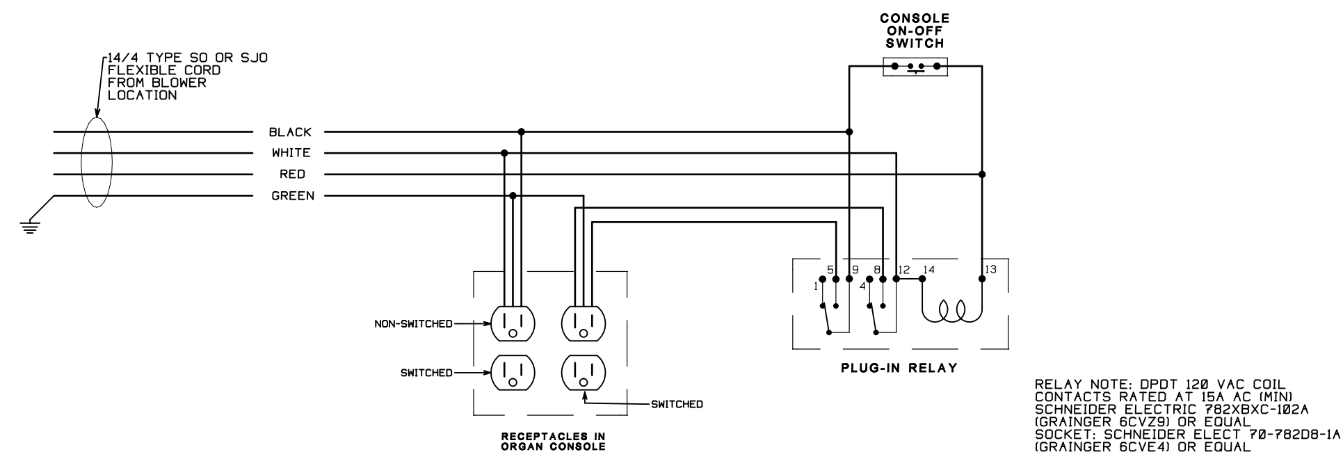
CONSOLE AC WIRING DIAGRAM
