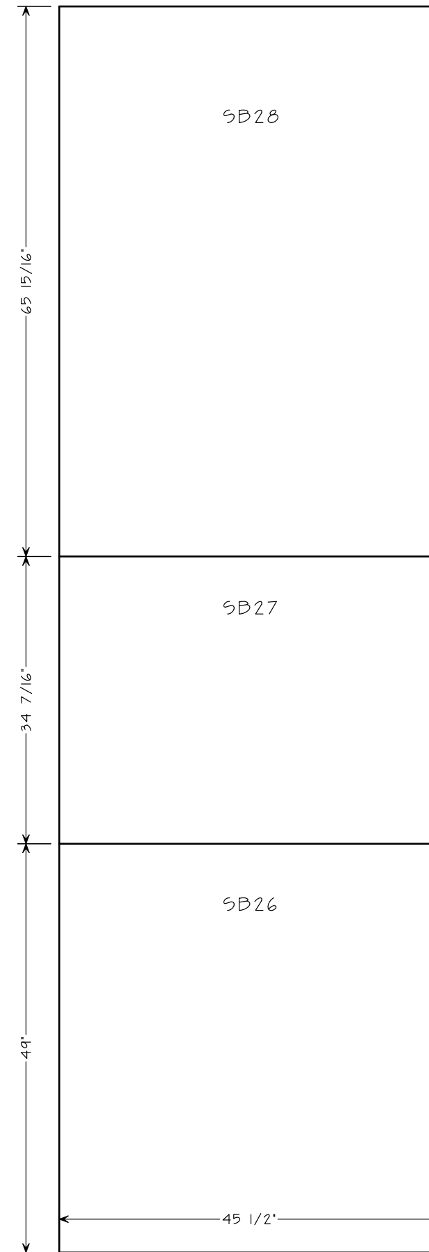
1 9 SW BOX PANEL DETAIL AT SOLO RIGHT FRONT SCALE 3/4" = 1' 0"
