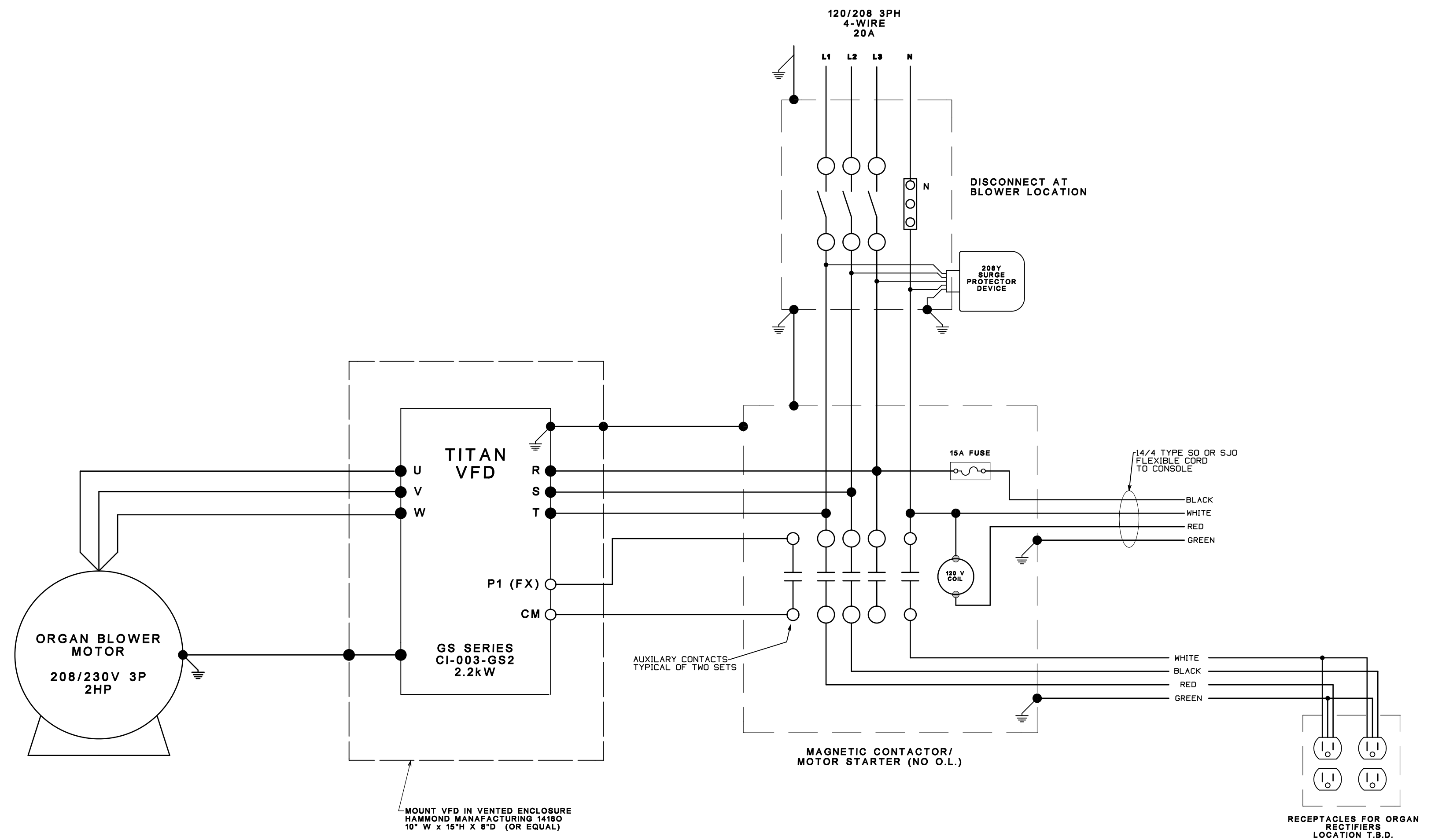
ORGAN AC CONTROL WIRING DIAGRAM
