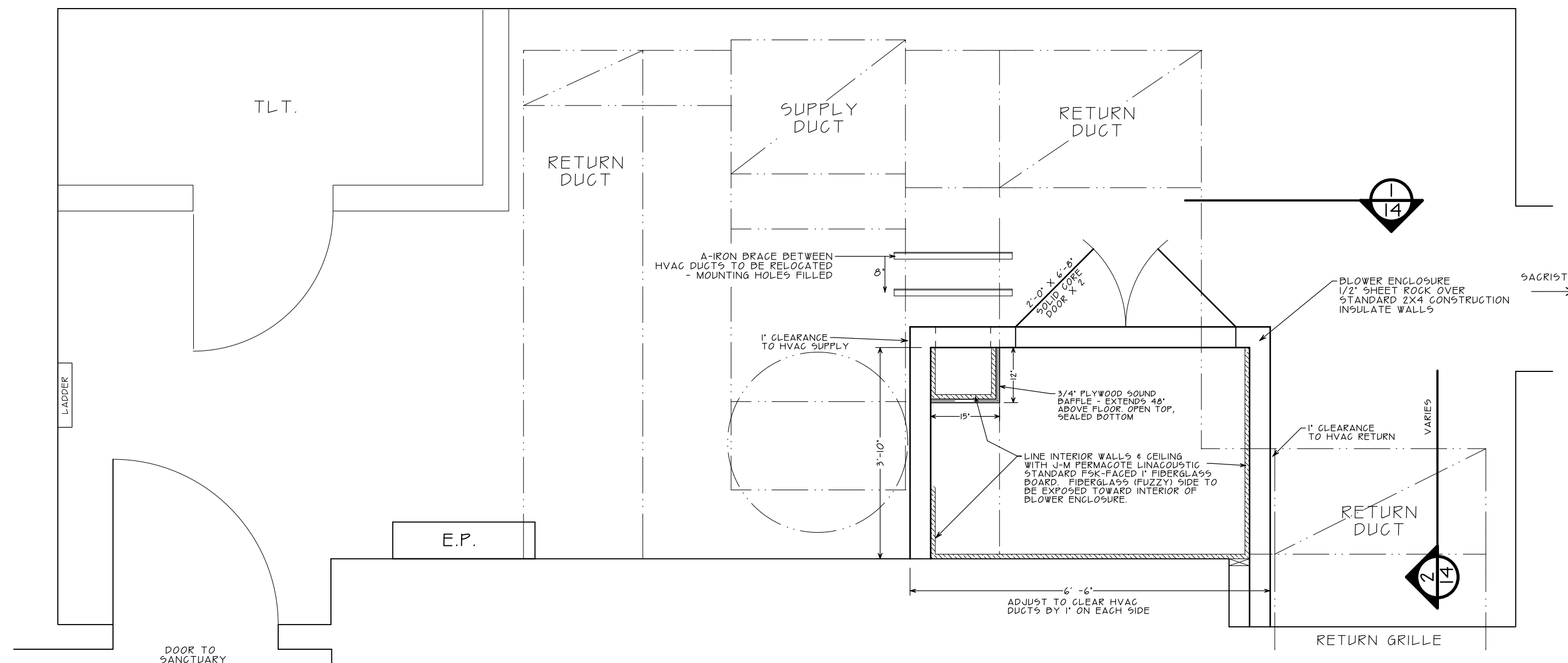
BLOWER ENCLOSURE ROOM PLAN
