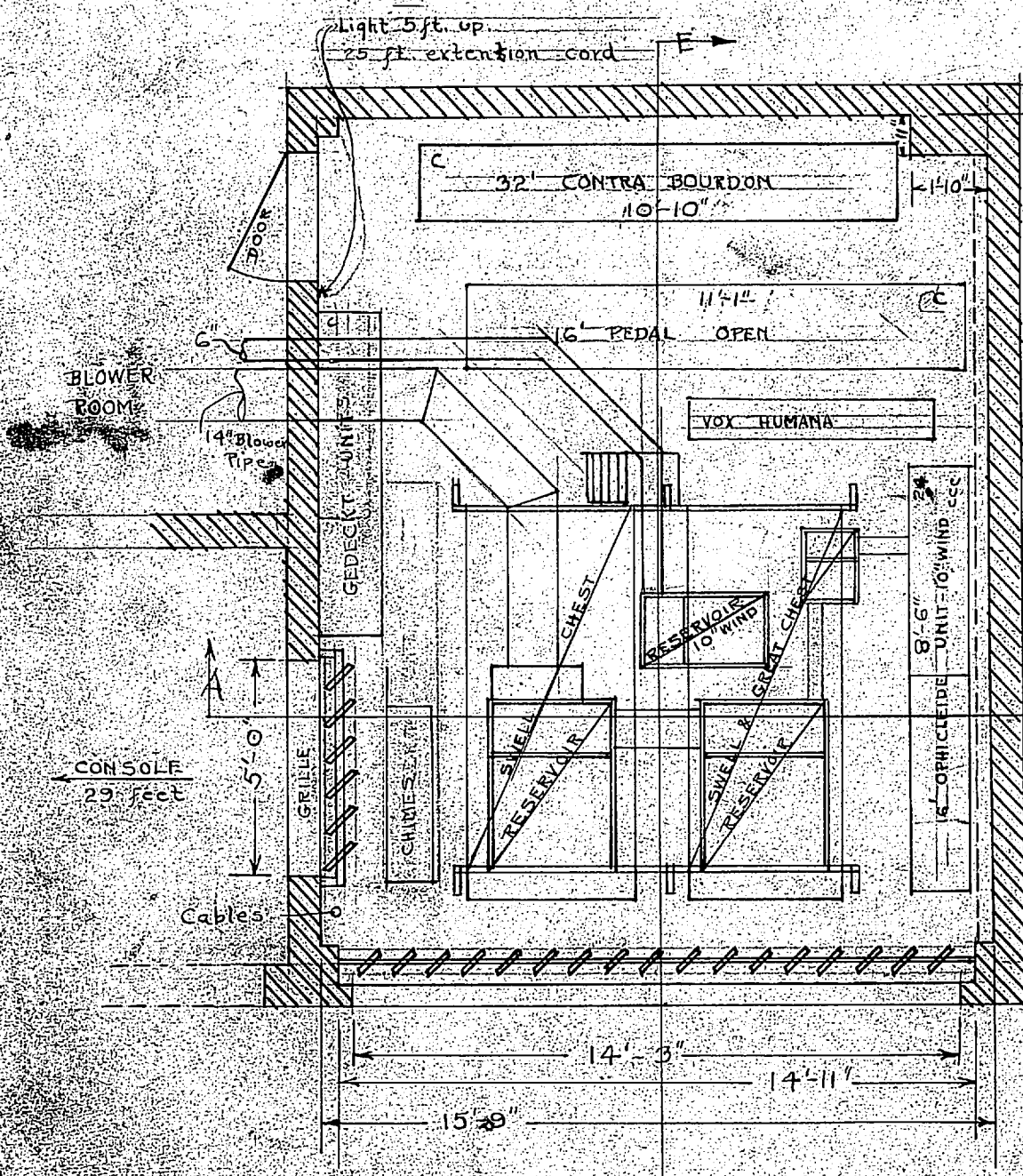
PLAN
