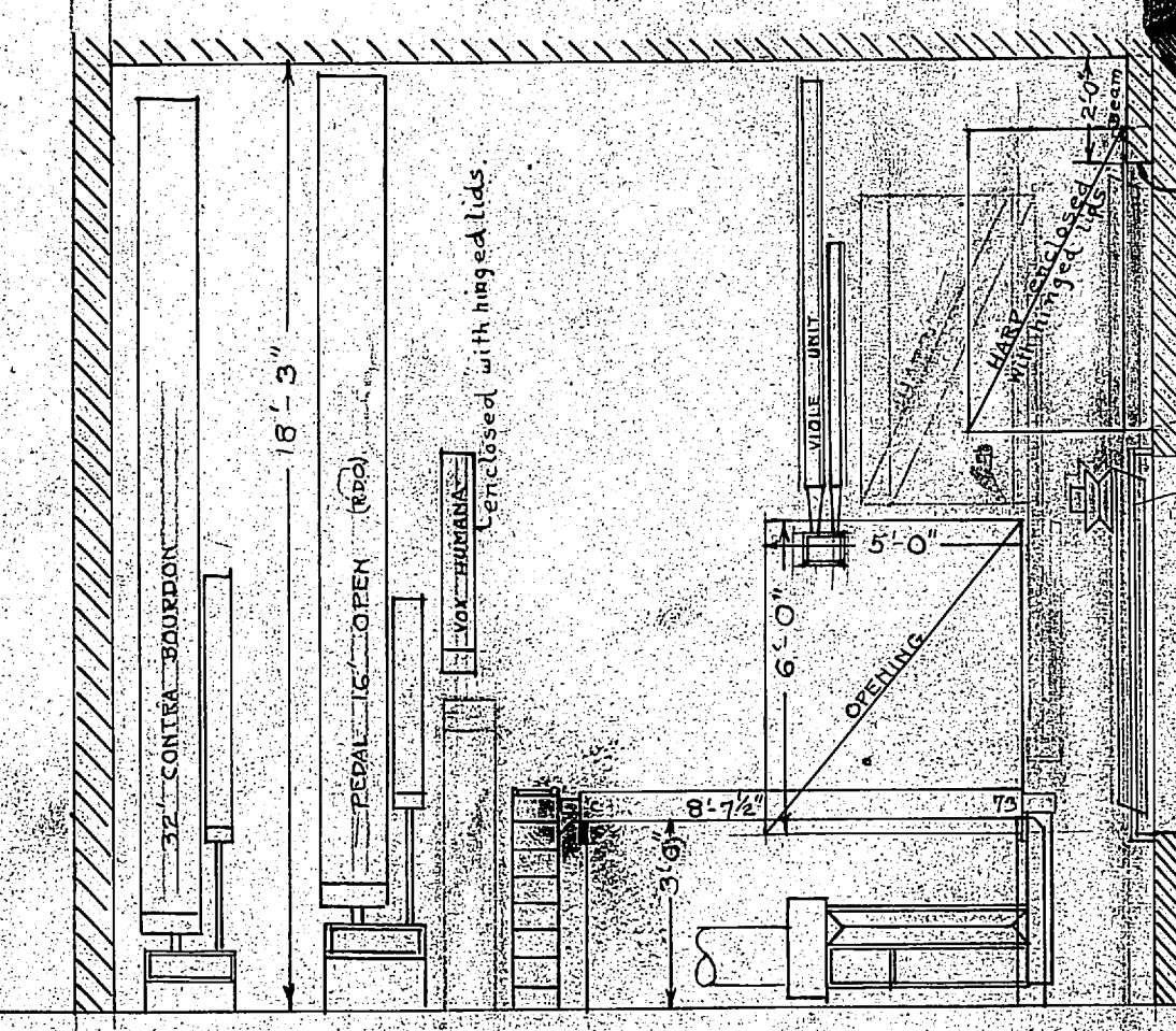
SECTION-EE
