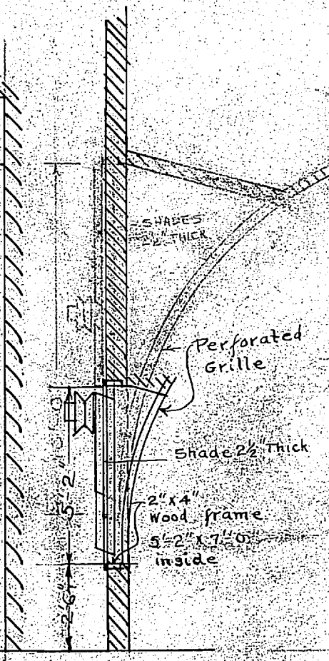
SECTION-DD
