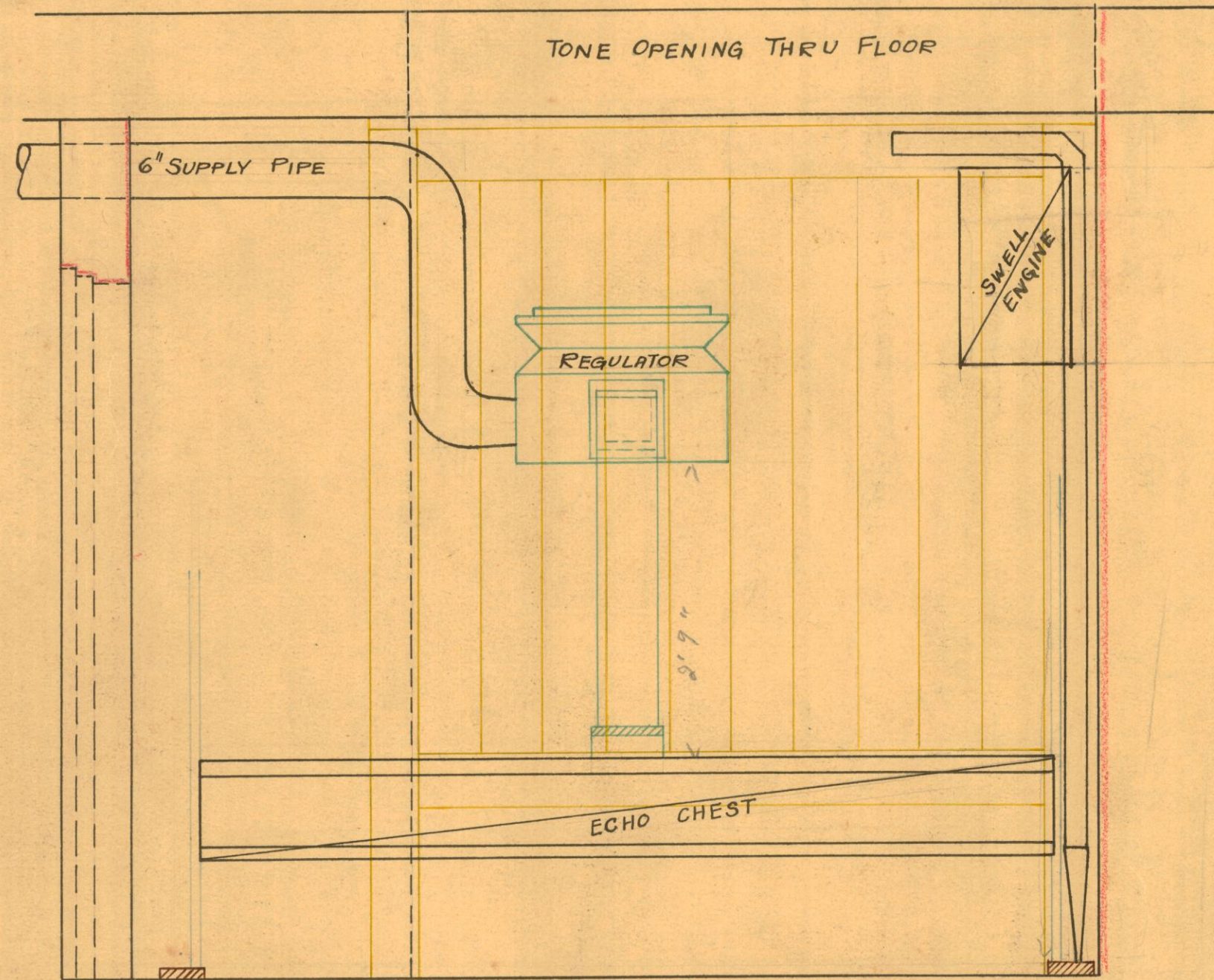
Front Elevation
