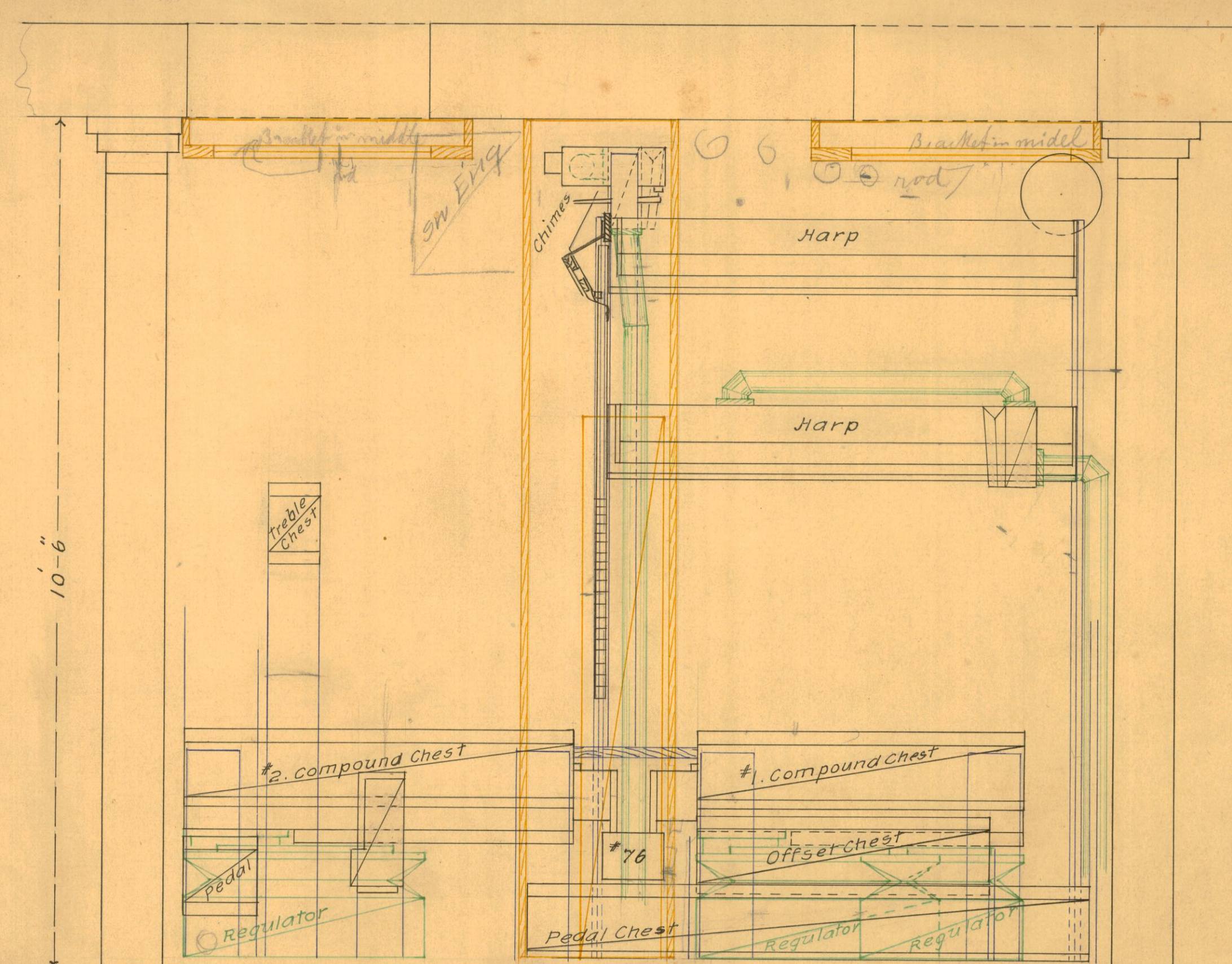
Front Elevation
