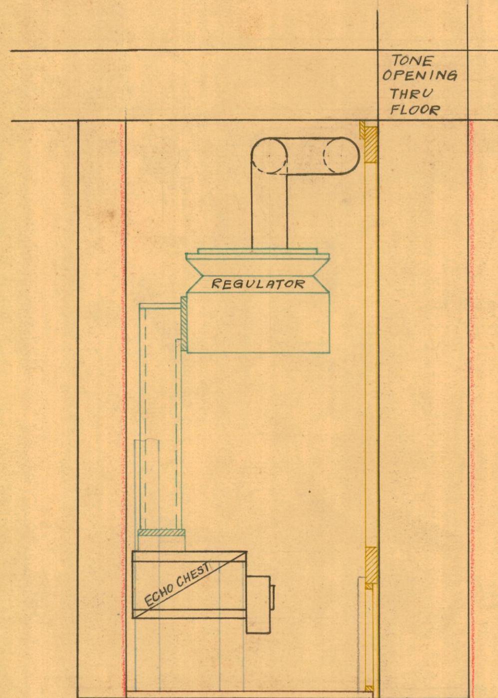
Section
