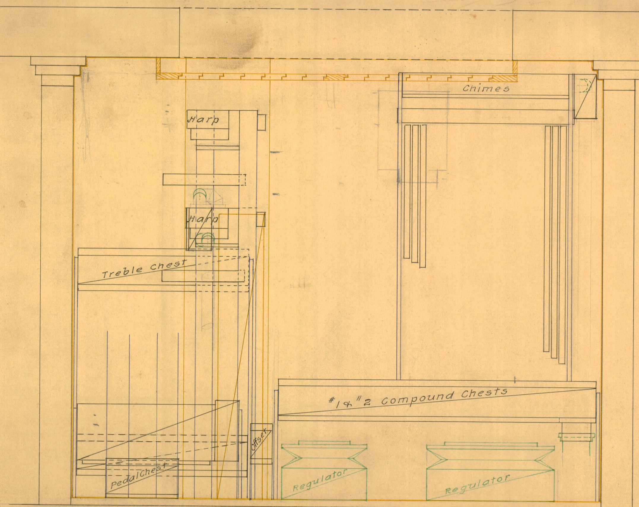
Section
