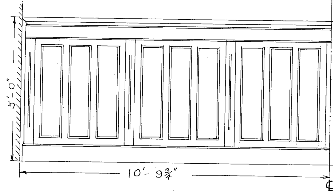
Scale-1/2"=1'-0"
