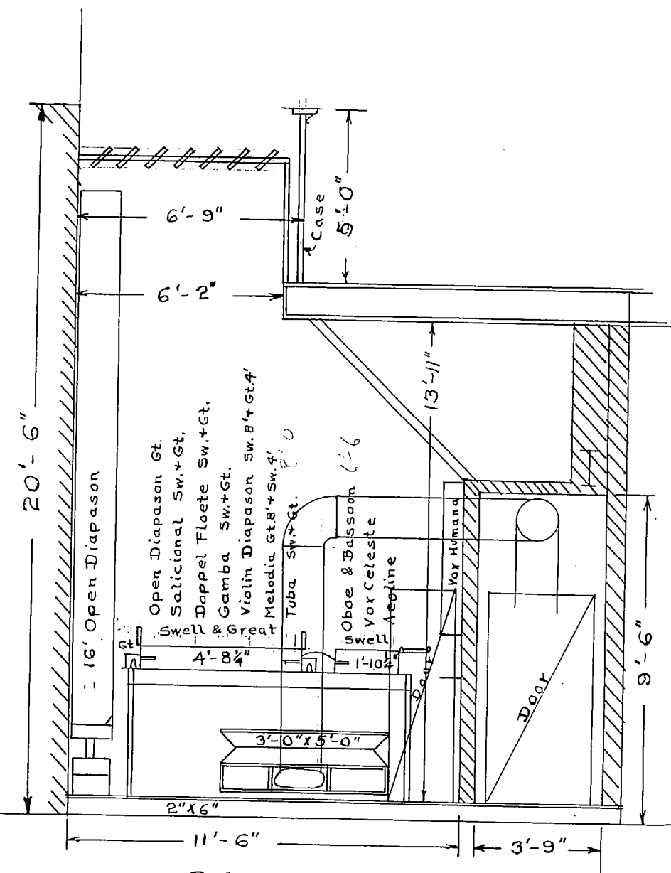
SECTION-BB
