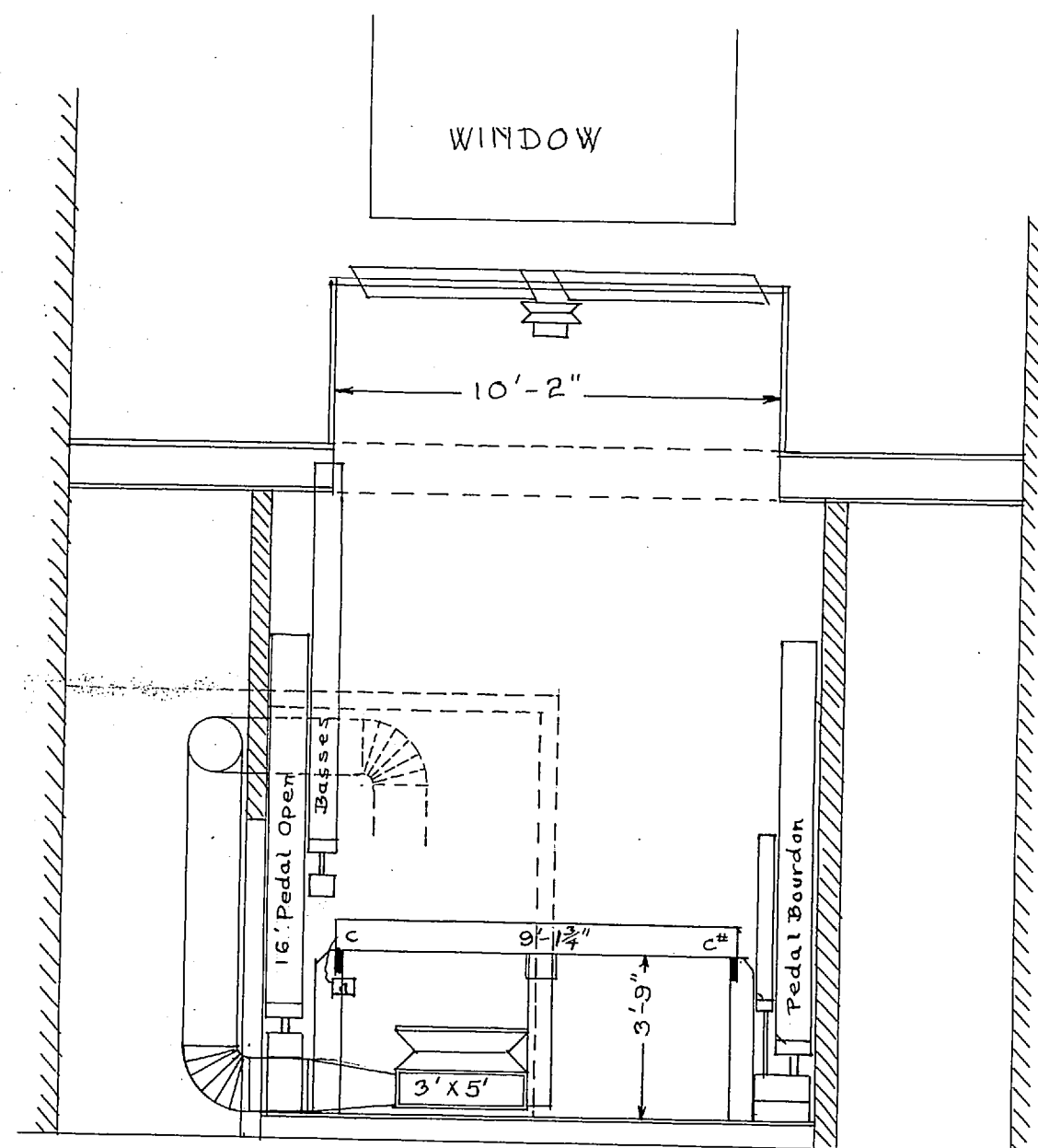
SECTION-AA
