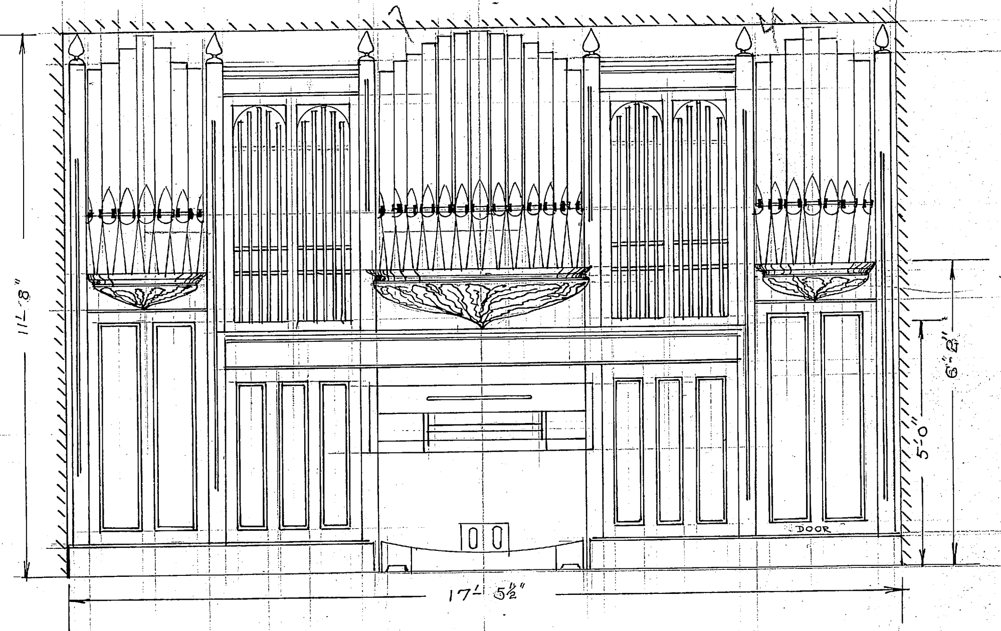
FRONT VIEW
