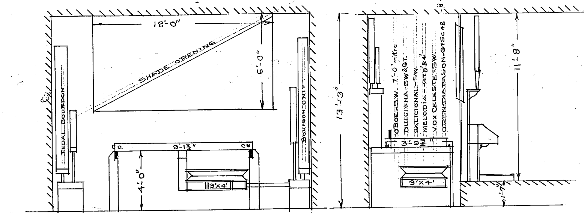
SECTION-BB
