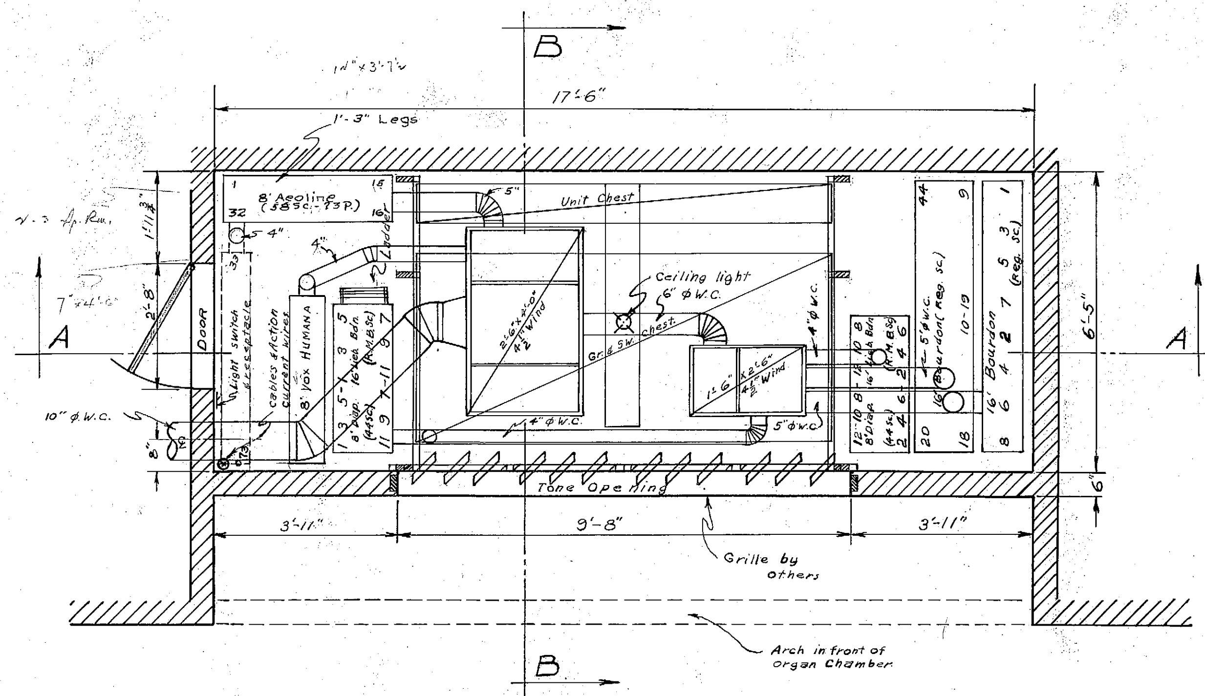
FLOOR PLAN
