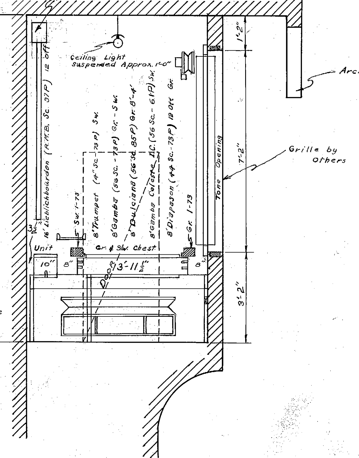
SECTION-BB
