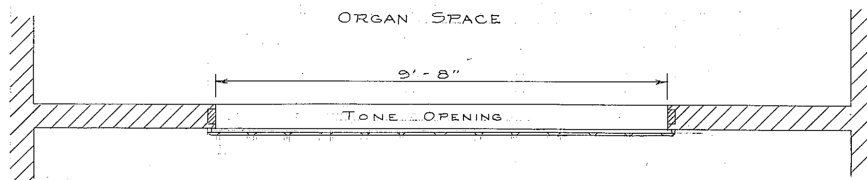
PLAN
