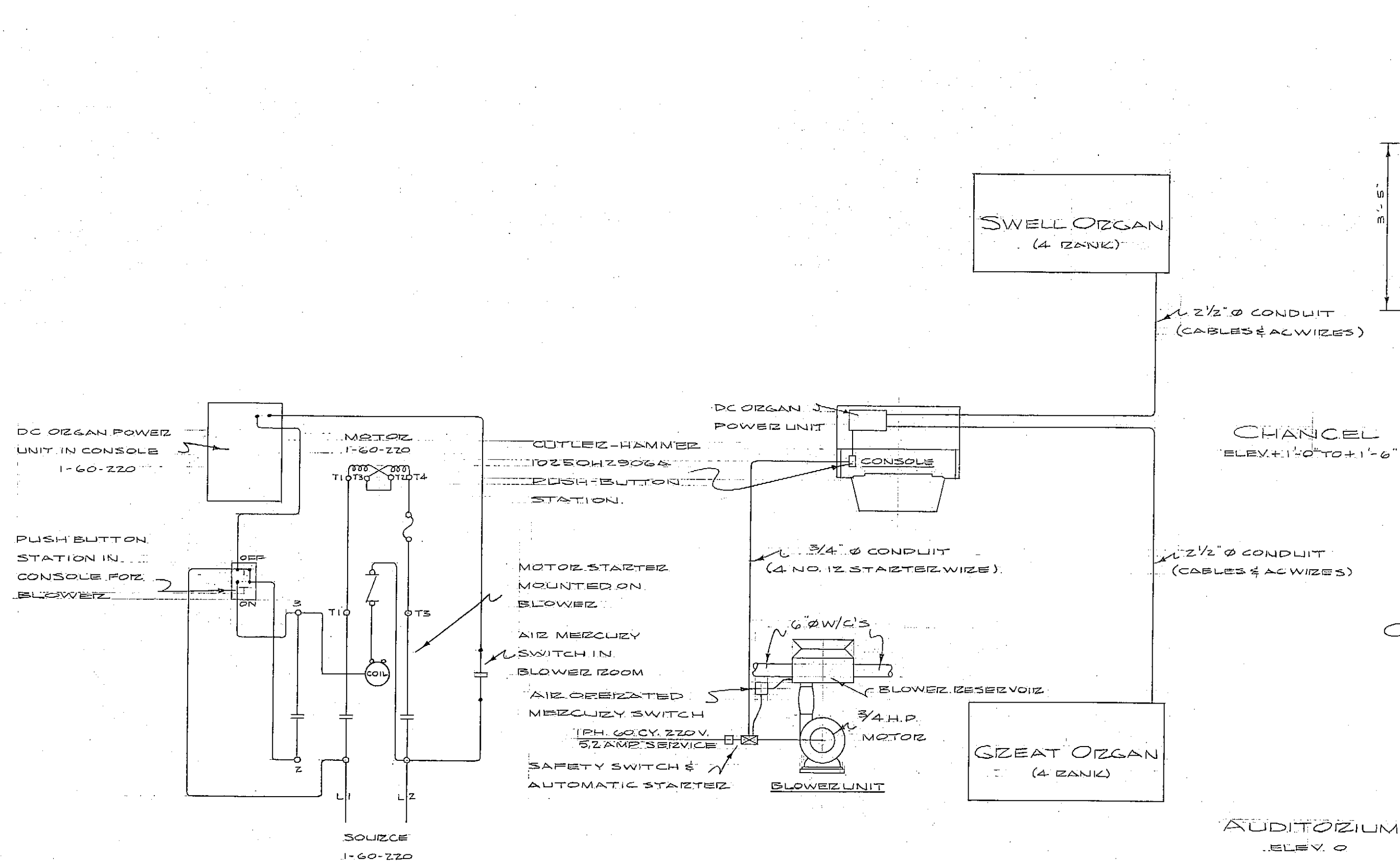
WIRING SCHEMATIC FOR DC ORGAN POWER UNIT
