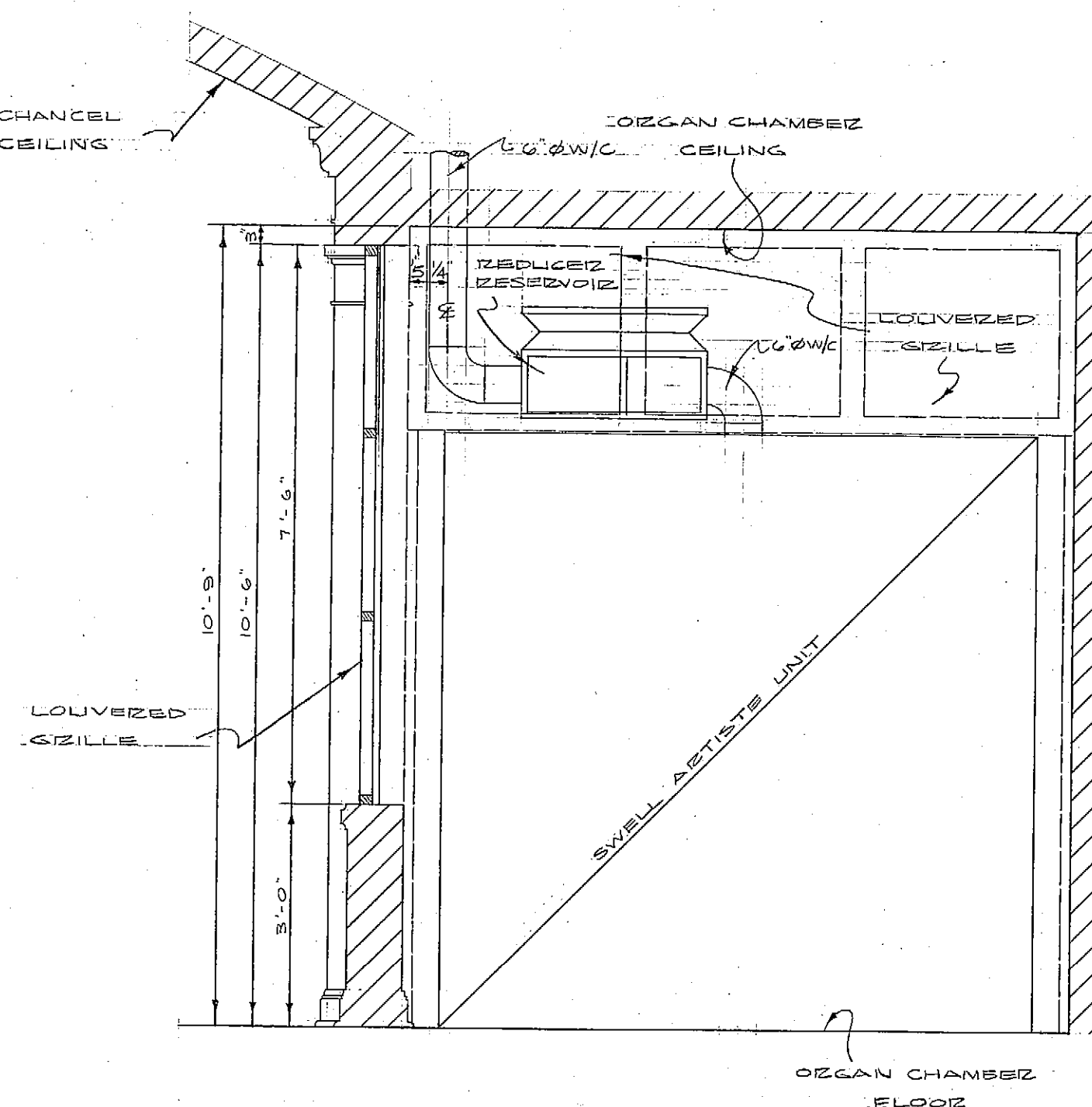
SECTION-AA
