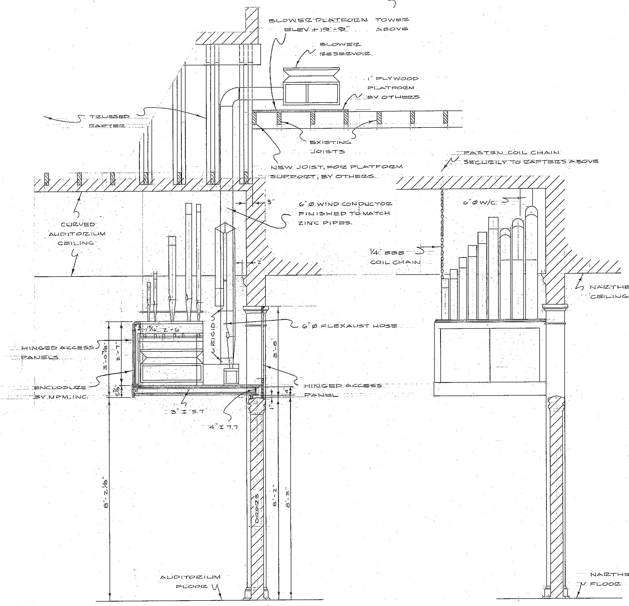
END VIEW OF ENCLOSURE
