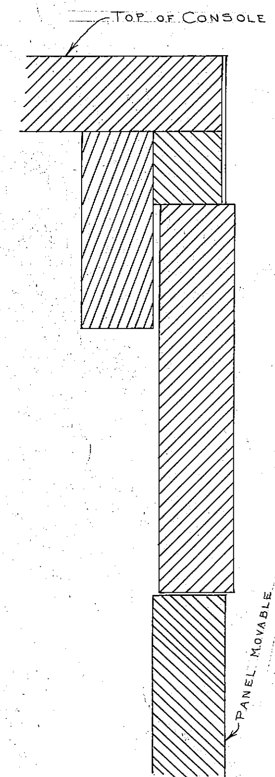
FULL SIZE DETAIL OF TOP AND SIDE OF CONSOLE
