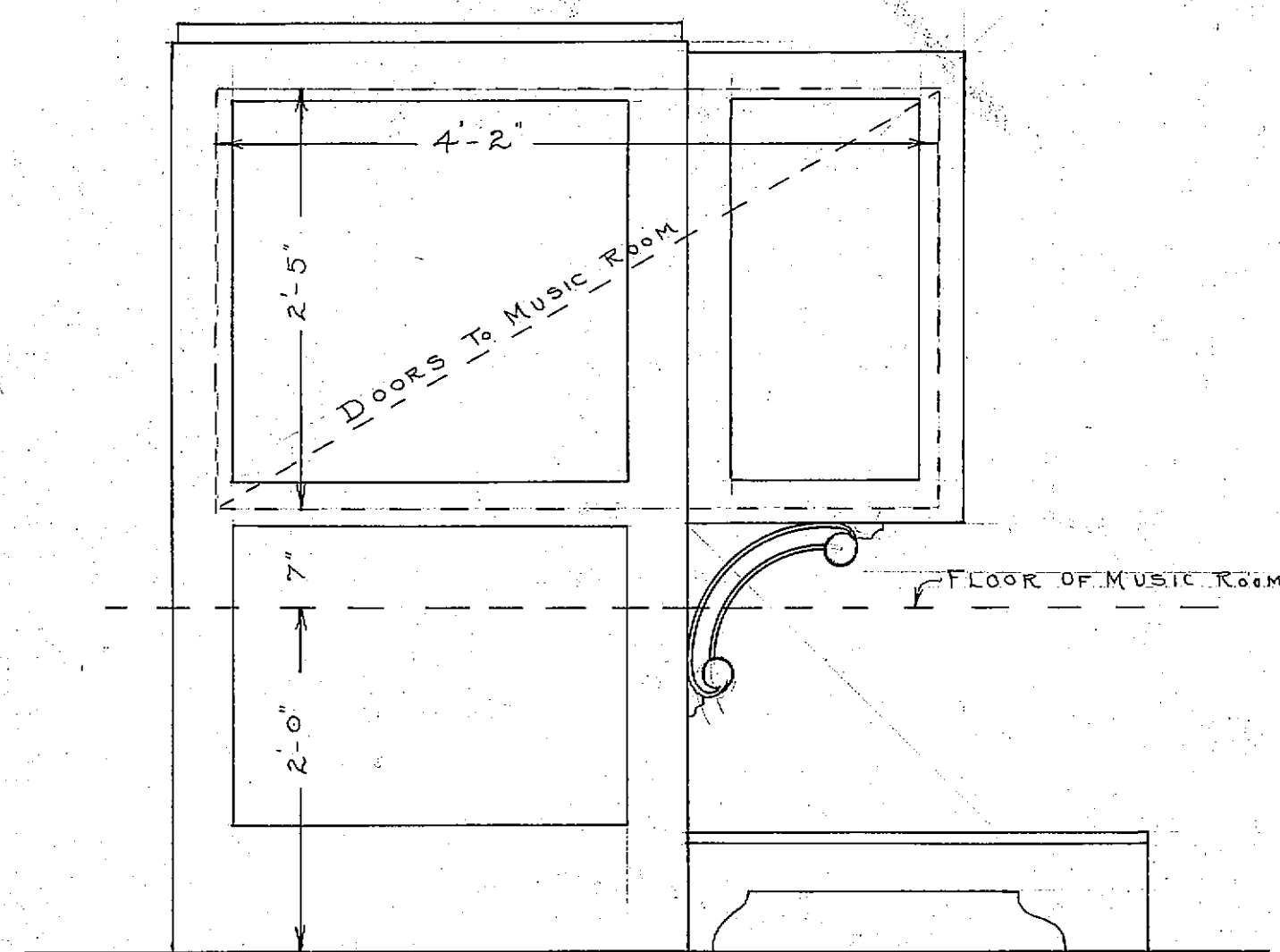
SECTION-CC
