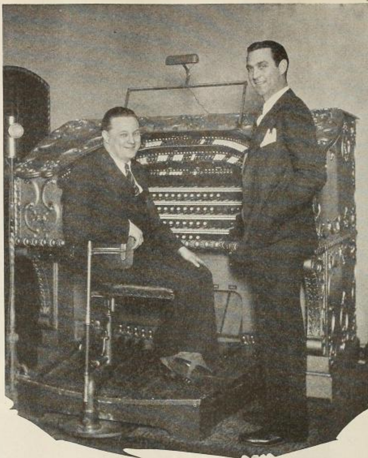
Magnificent console of Page DeLuxe Unit Organ installed in W-H-T, the broadcasting studio of The Radiophone Broadcasting Corporation, in the Wrigley Building, Chicago, Ill.
