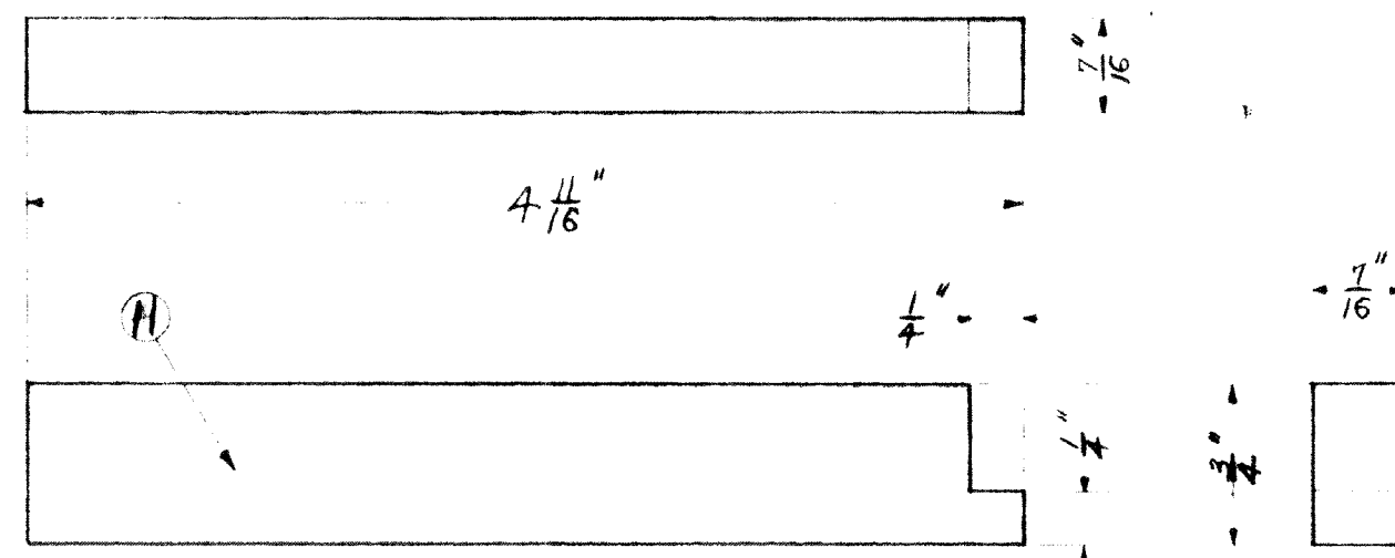
FRAME END.
