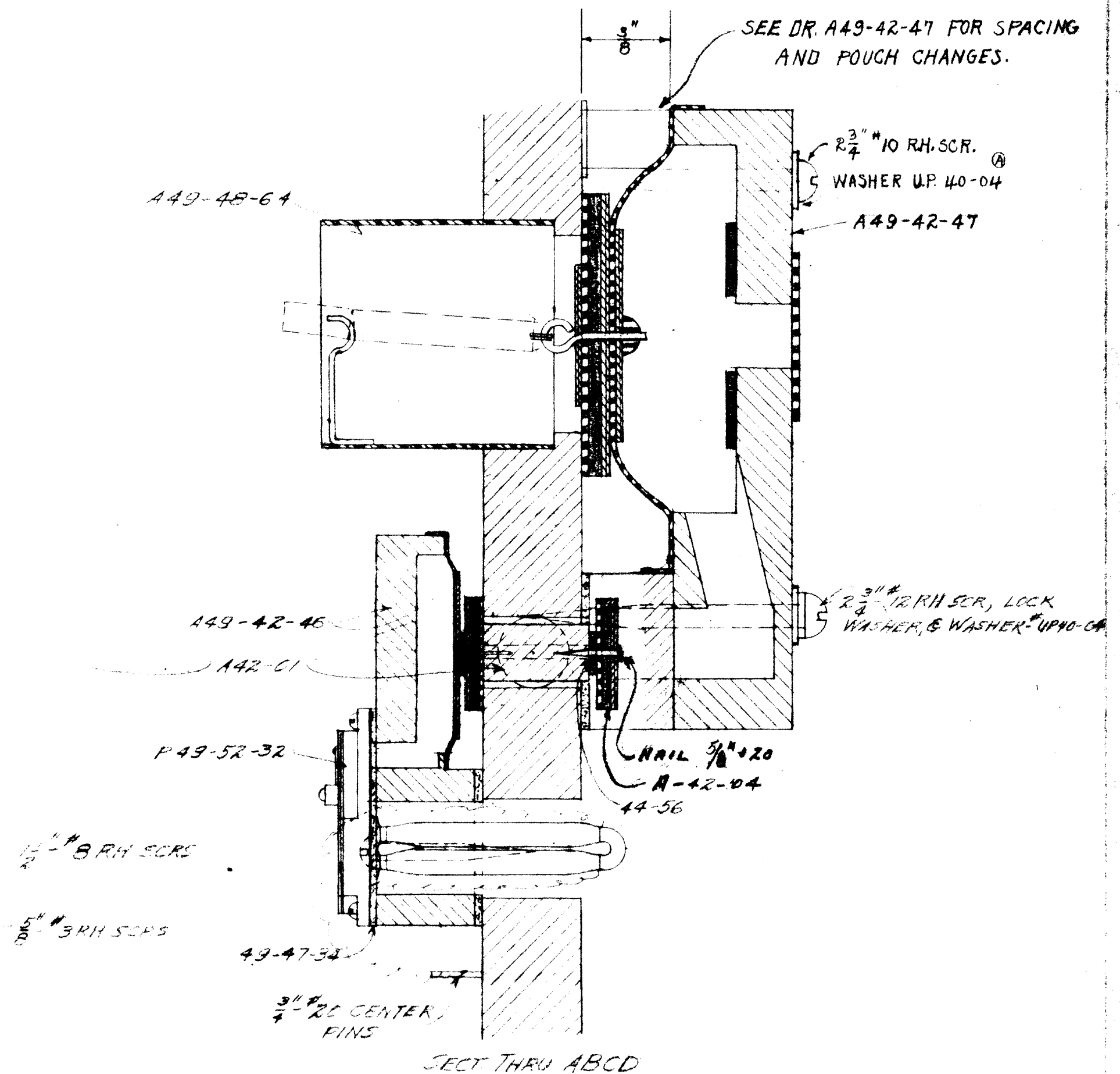
SHOWING ARRANGEMENT OF PRIMARY & SECONDARY VALVES ON PEDAL PIPE CHEST.
