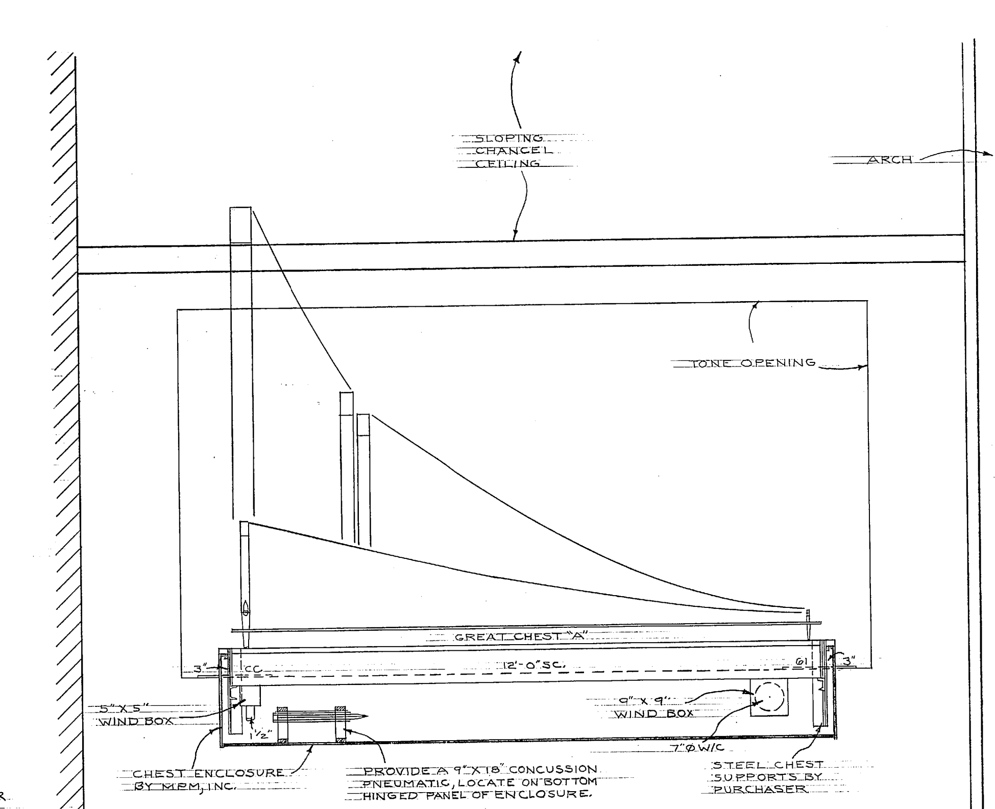
SECTION THRU EXPOSE GREAT CHEST "A"
