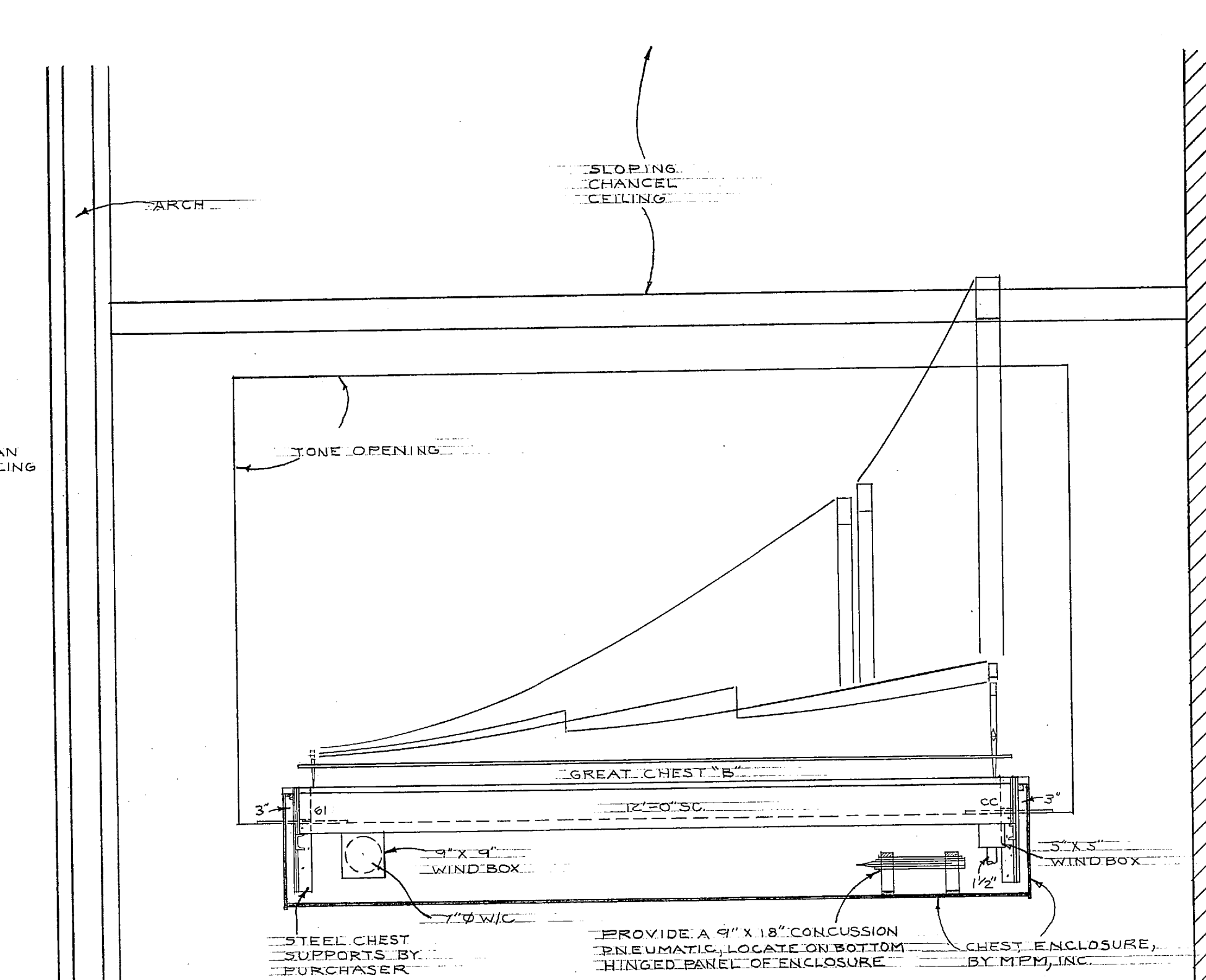
SECTION CC
