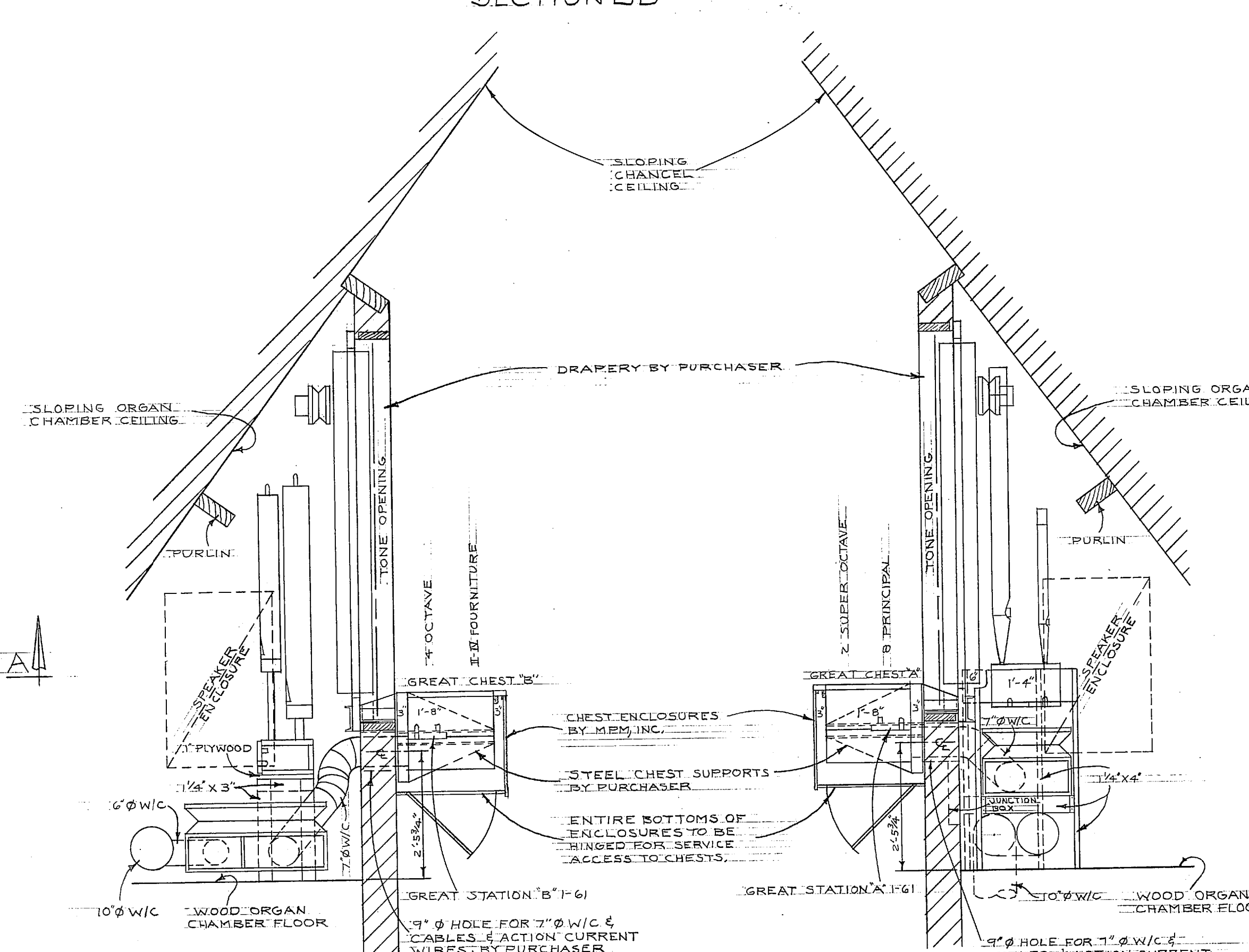
SECTION E
