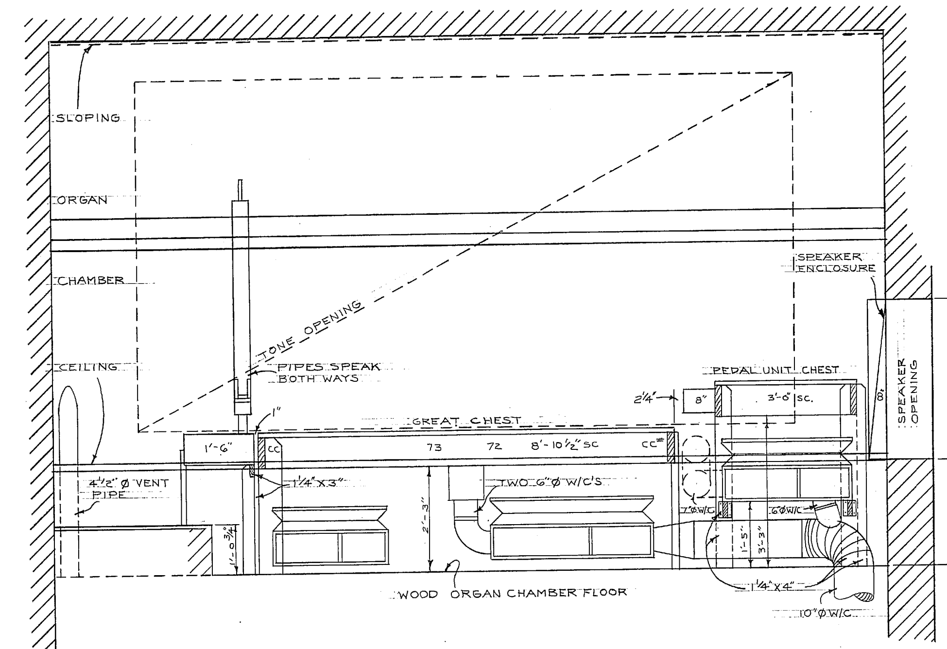
SECTION CC
