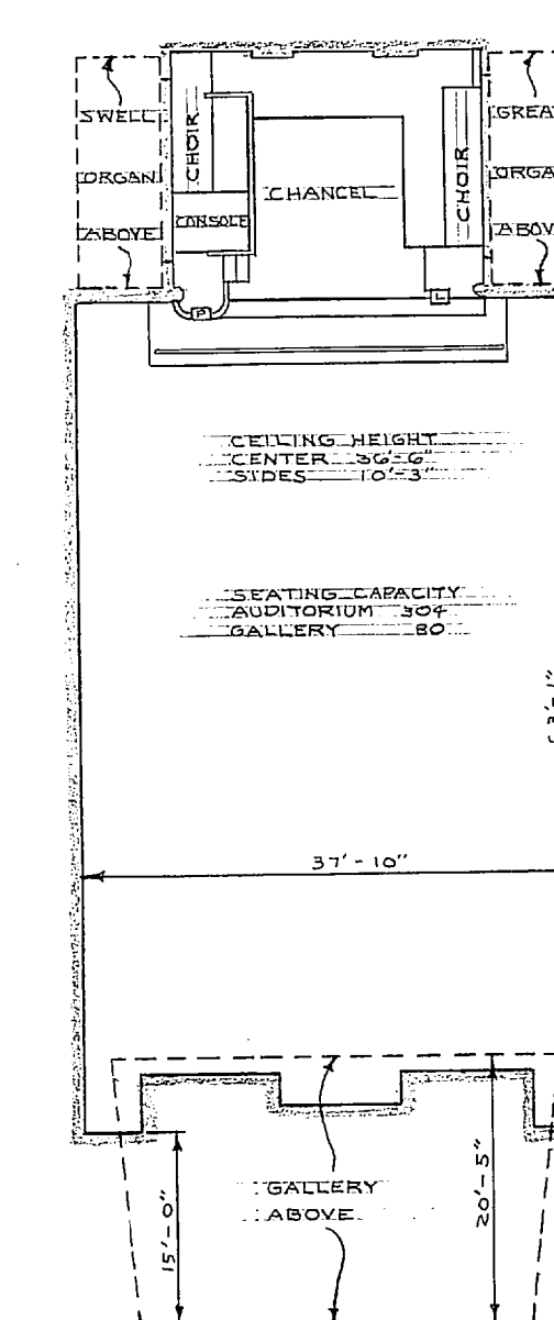
AUDITORIUM PLAN SCALE=1/4"=1'-0"
