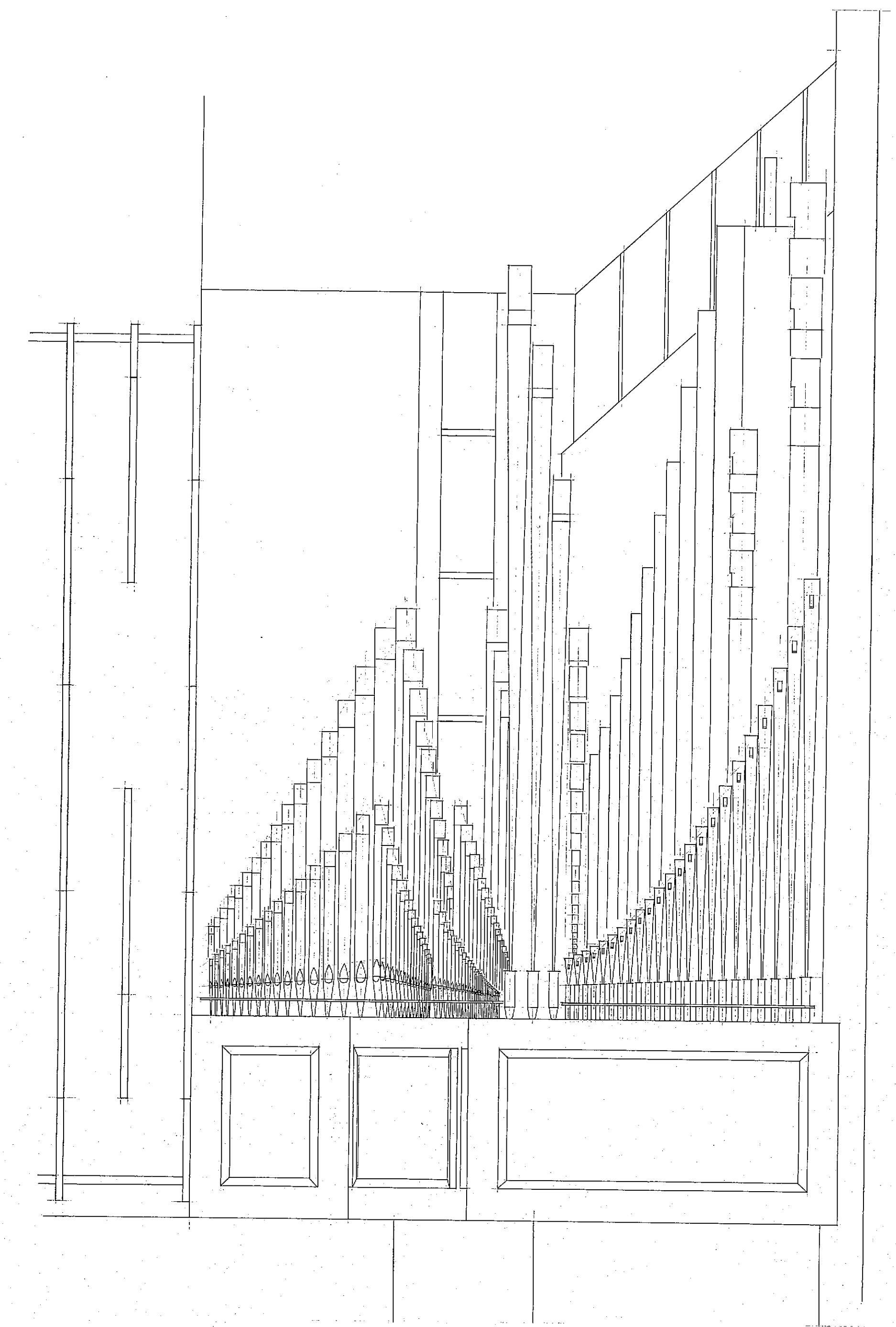
• SIDE ELEVATION •
