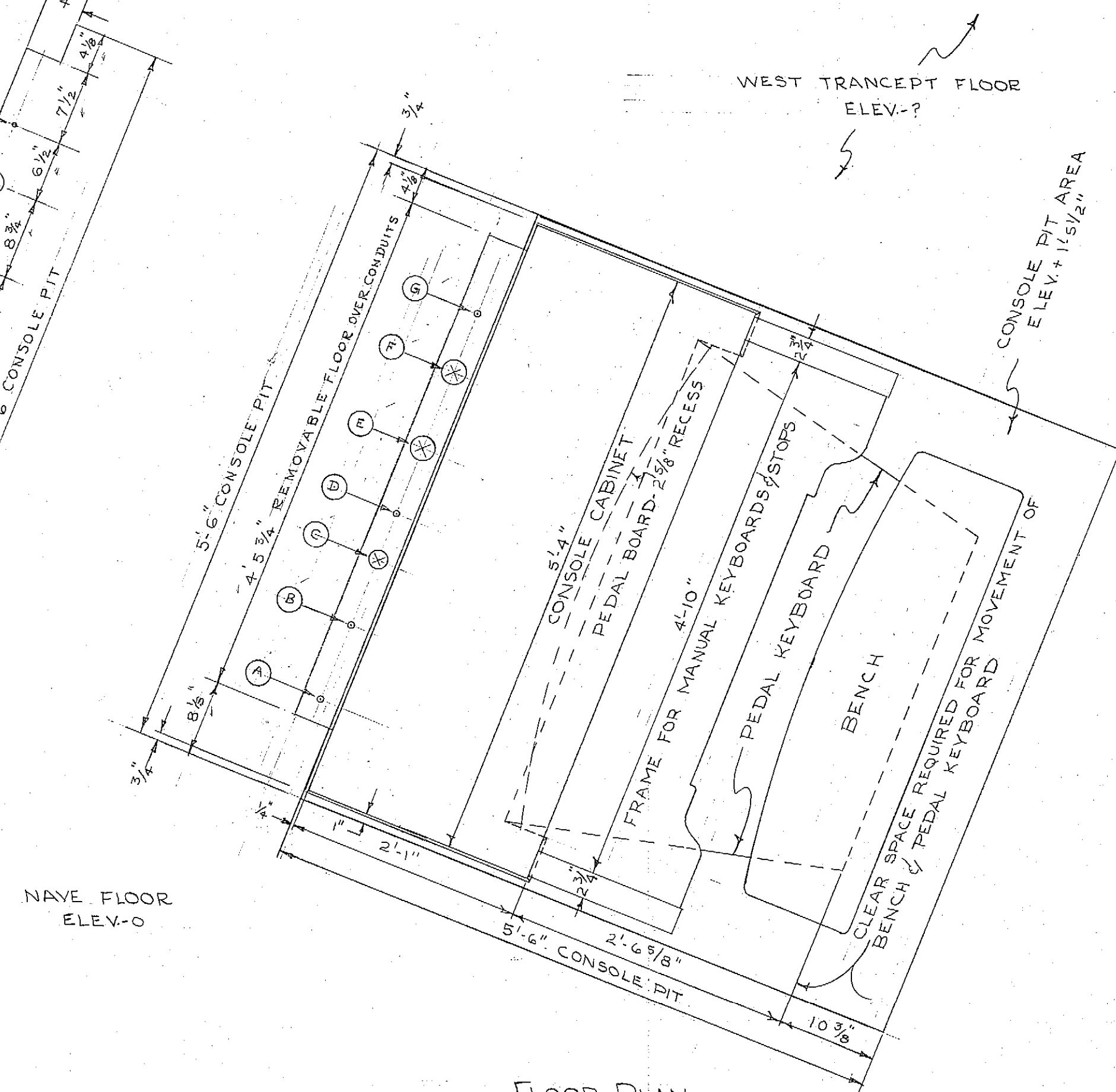
FLOOR PLAN
