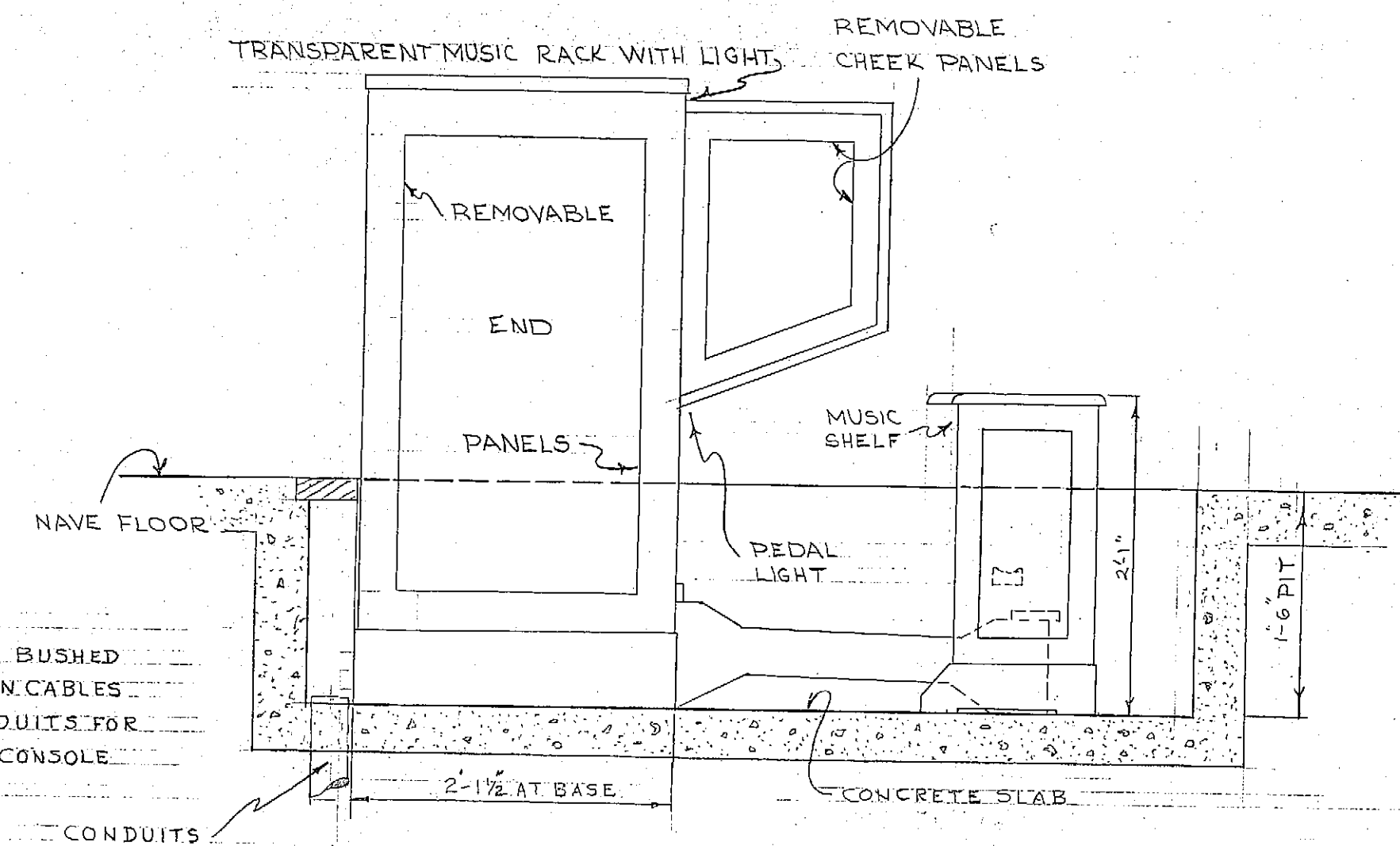
END VIEW
