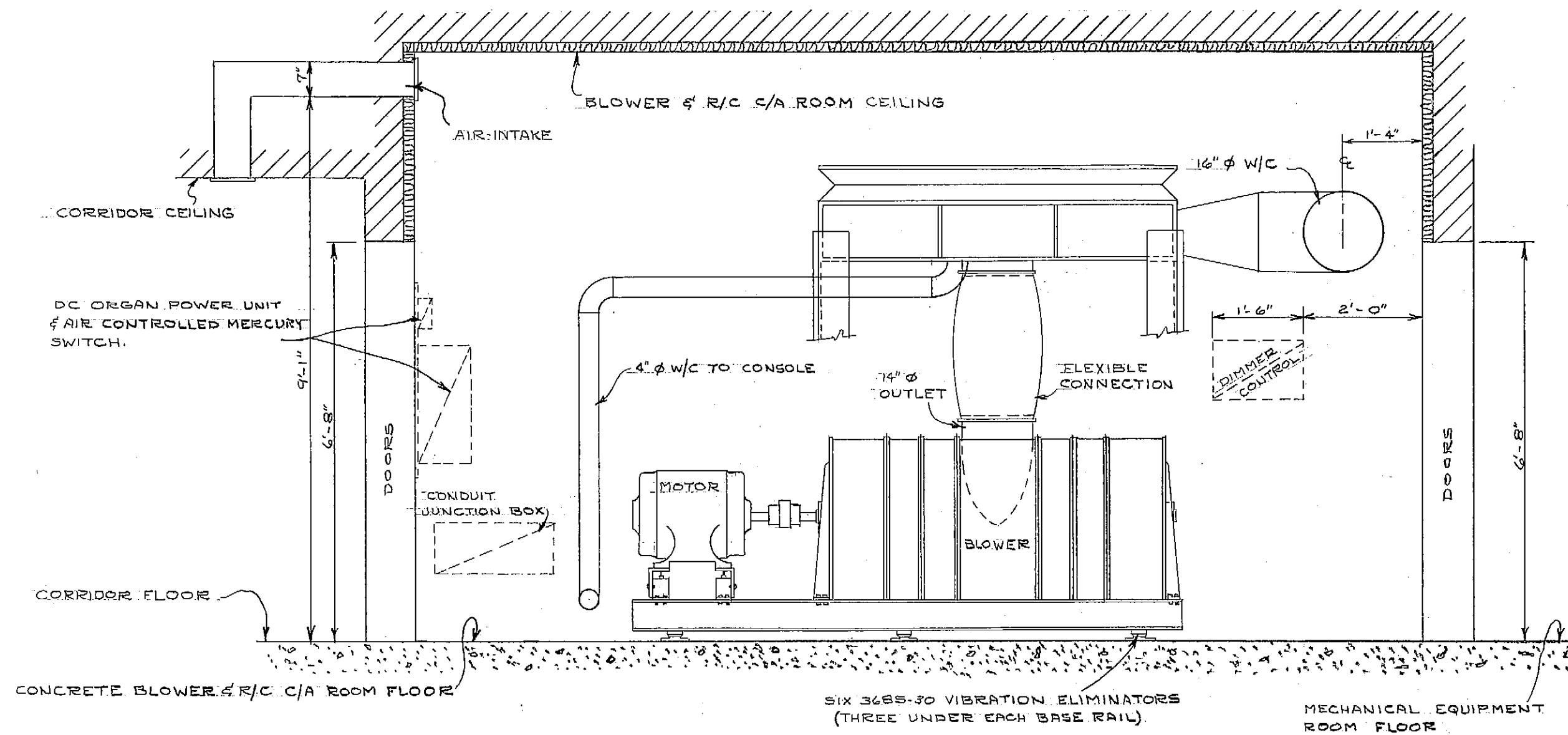
SECTION BB
