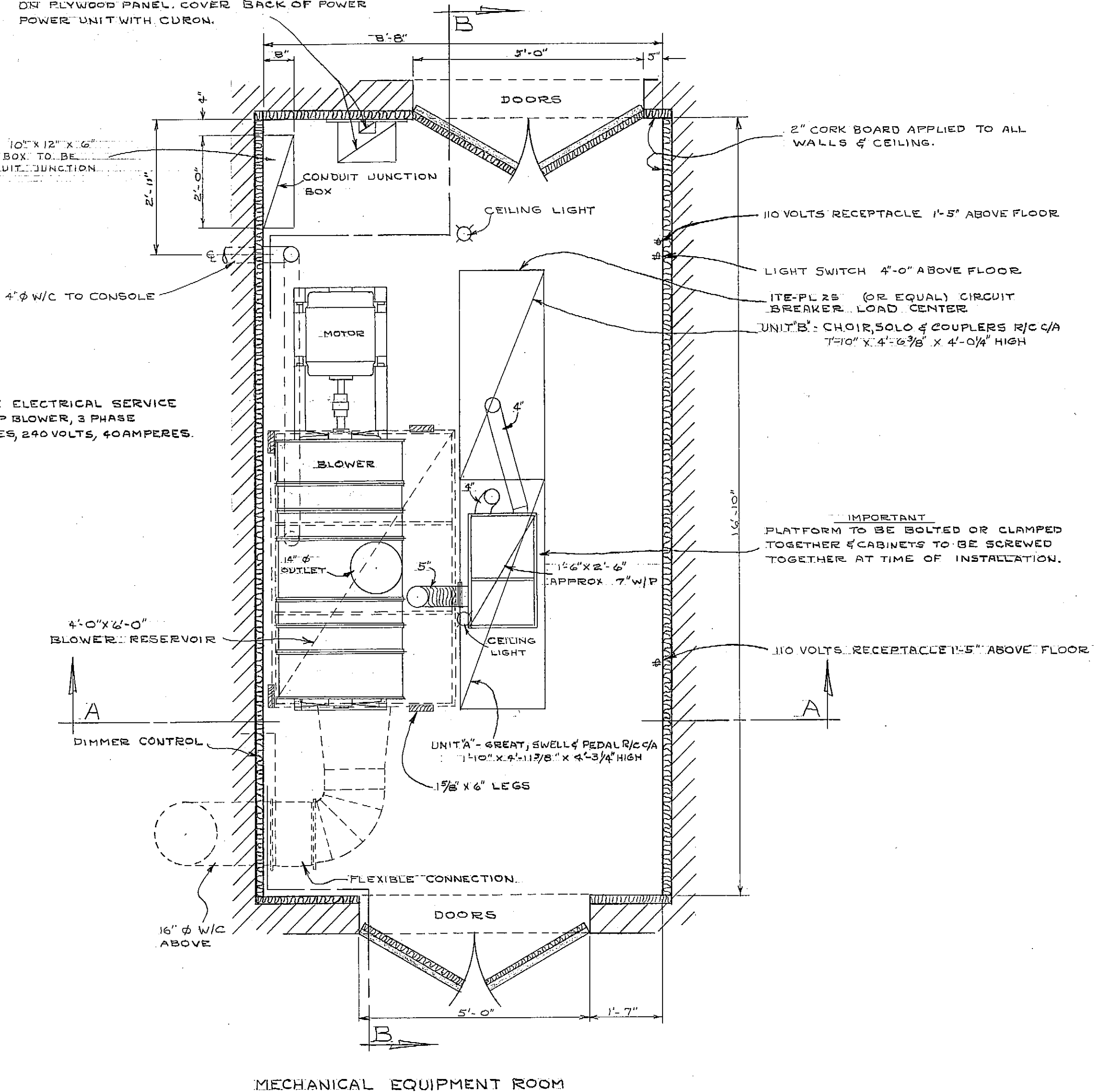
FLOOR PLAN
