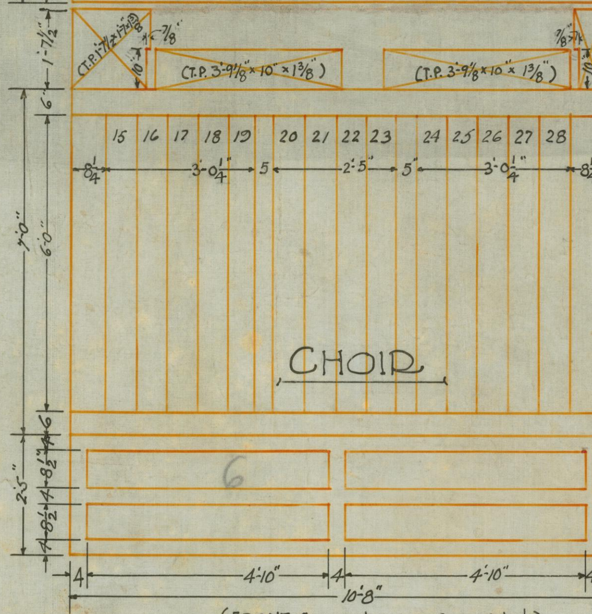
(FRONT ELEV. Looking from outside)
